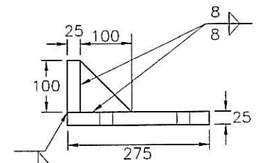
ANGLE DETAIL 1:10
