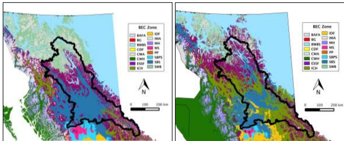
Figure 2. Current (BEC version 8) and projected future (2041-2070) BEC zone locations. Future map shows consensus of multiple projections. Maps from ClimateBC .
