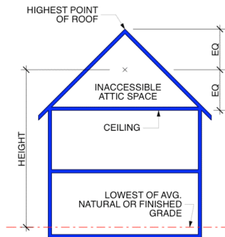
PITCHED ROOFS w/ ATTIC SPACE
