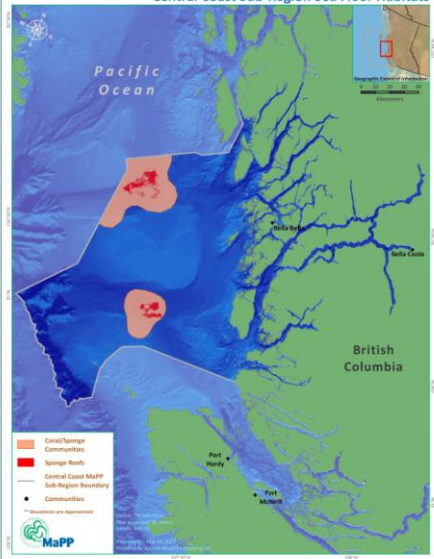
Central Coast Sub-Region Sea Floor Habitats
