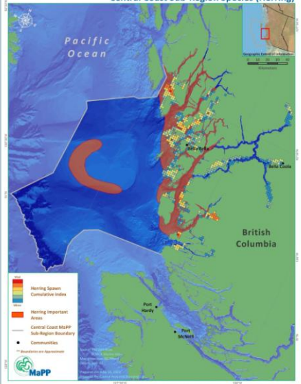
Central Coast Sub-Region Species (Herring)
