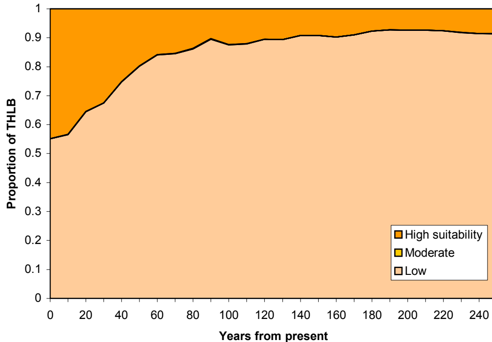
Figure 14. Mountain caribou habitat suitability for the early winter season on the timber harvesting land base of the Arrow Timber Supply Area. Habitat suitability is projected from 10-250 years from present for the early winter season (25 October-15 January; Hamilton et al. 2000). Harvest scheduling was based on the Arrow IFPA's spatial timber supply analysis (Timberline 2002).
