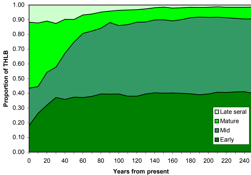
Figure 11. Seral distribution of stands on the timber harvesting land base of the Arrow Timber Supply Area. Seral distribution is projected from 10-250 years from present. Harvest scheduling was based on the Arrow IFPA's spatial timber supply analysis (Timberline 2002).
