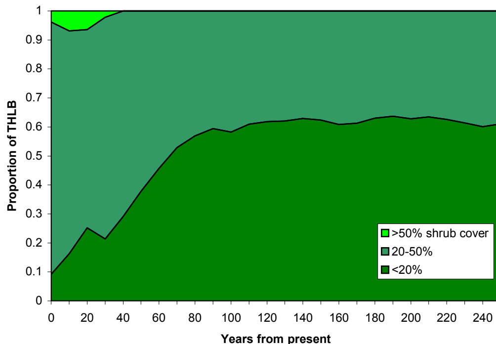
Figure 10. Percent shrub cover on the timber harvesting land base of the Arrow Timber Supply Area. Shrub cover is projected from 10-250 years from present. Harvest scheduling was based on the Arrow IFPA's spatial timber supply analysis (Timberline 2002).
