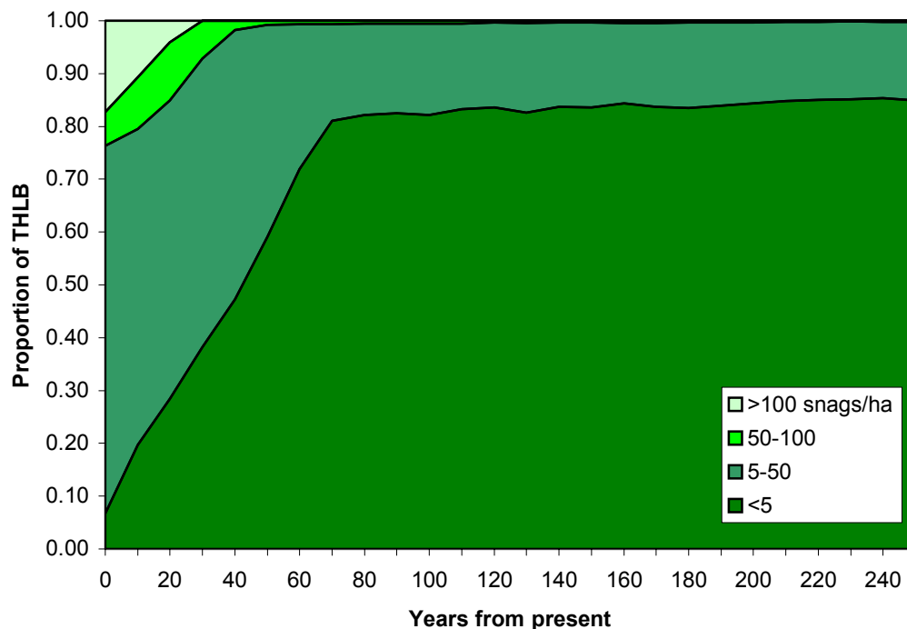
Figure 7. Snag densities ( >30 \text{ cm dbh} ) on the timber harvesting land base of the Arrow Timber Supply Area. Densities are projected from 10-250 years from present. Harvest scheduling was based on the Arrow IFPA's spatial timber supply analysis (Timberline 2002).
