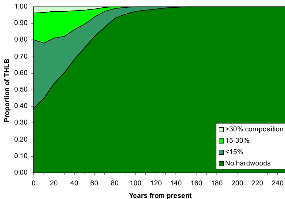
Figure 9. Percent composition of hardwoods on the timber harvesting land base of the Arrow Timber Supply Area. Composition is projected from 10-250 years from present. Harvest scheduling was based on the Arrow IFPA's spatial timber supply analysis (Timberline 2002).
