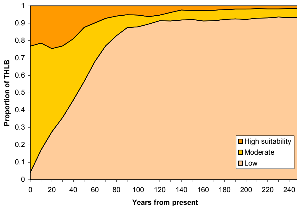
Figure 13. Pileated woodpecker habitat suitability on the timber harvesting land base of the Arrow Timber Supply Area. Habitat suitability is projected from 10-250 years from present. Harvest scheduling was based on the Arrow IFPA's spatial timber supply analysis (Timberline 2002).
