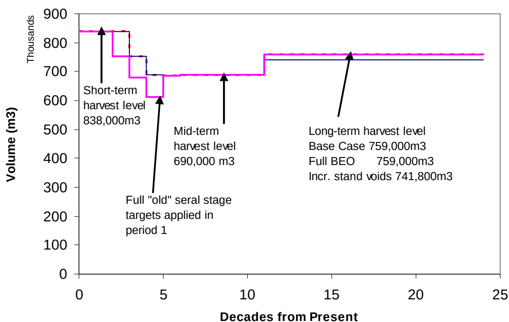
Figure 29 Harvest flows from wildlife strategies
