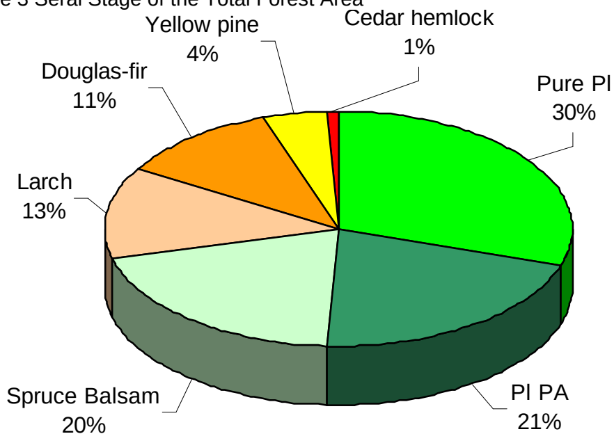
Figure 3 Seral Stage of the Total Forest Area
