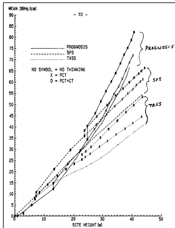
Figure 7. Model Comparison, Interior Douglas-fir
