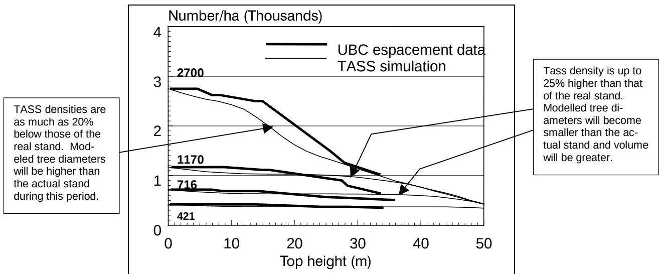
Figure 2. TASS Douglas-fir Validation, Haney Plots
