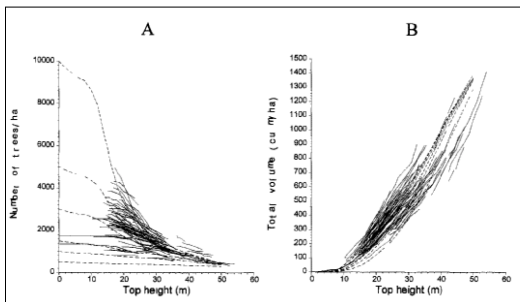
Figure 6. Example of a TASS Calibration
