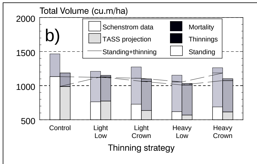
Figure 3. Douglas-fir Validation, Schenstrom Plots
