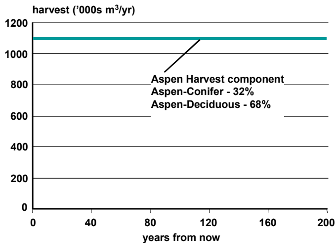
Figure A2-9. Aspen harvest forecast, Fort Nelson TSA, 1992
