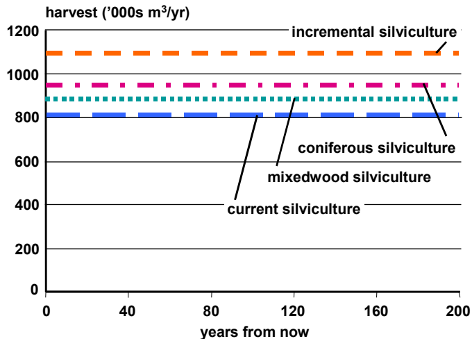
Figure A2-5. Sensitivity of the coniferous harvest component to silviuctural activities, Fort Nelson TSA, 1992
