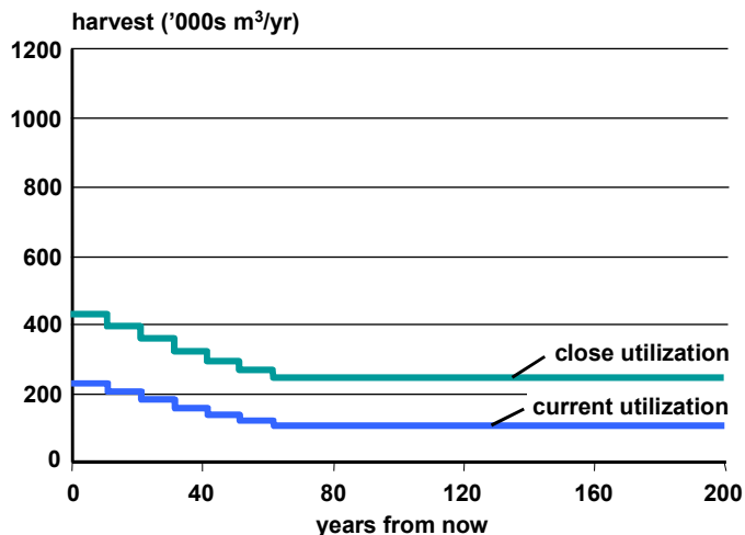
Figure A2-8. Sensitivity to alternate utilization standards on the aspen harvest forecast, Fort Nelson TSA, 1992
