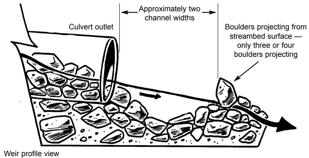
Figure 10. Typical downstream weir.
