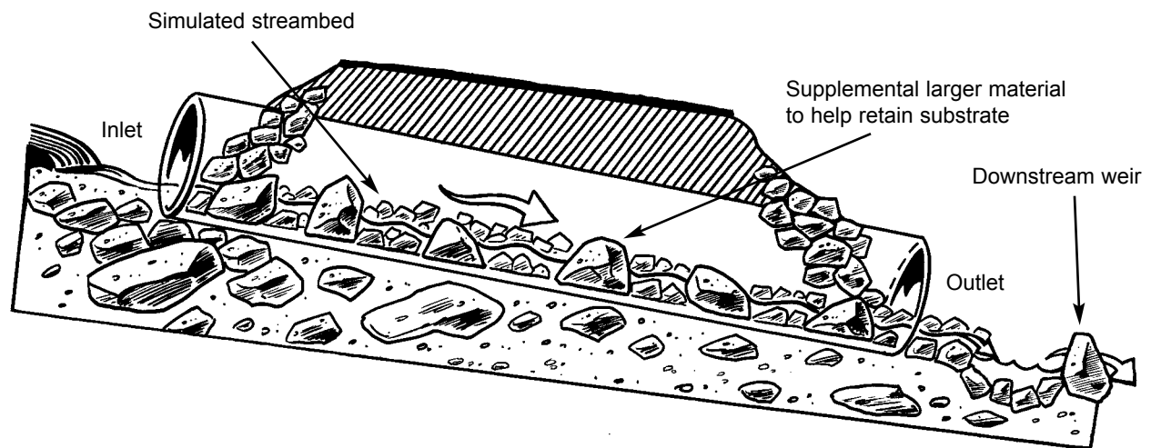
Figure 7. Typical closed bottom structures.
