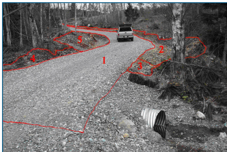
Photograph 2. Upstream view of a culvert crossing on an S6 stream. Like Photograph 1, the red lines and numbers delineate areas that are similar with respect to the amount of bare erodible ground exposed and the degree of hydrological connectivity to the stream.
