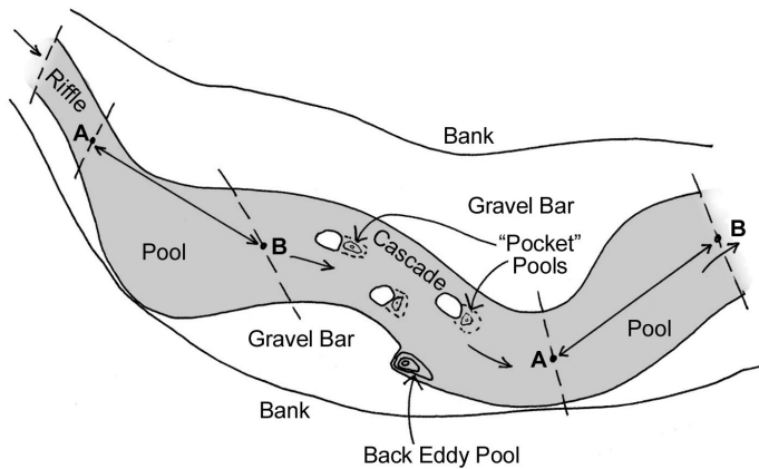
Figure 6. This is a plan-view sketch of two pool-riffle/cascade sequences in a stream. To determine the length of the reach with pool habitat, only measure the length of the main pools that occupy the width of the wetted channel, not back eddies or small scour holes or "pocket" pools behind boulders. Measure the length of the main pools from A to B, the mid-points of the pool-riffle boundaries
