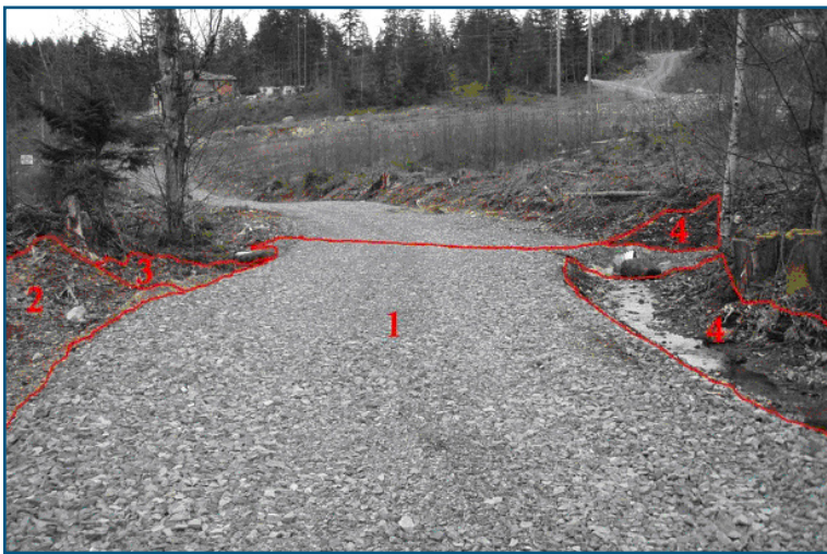
Photograph 1. Downstream view of a culvert crossing on an S6 stream. The stream flows down the right side ditch, then across the road from right to left. The red lines and numbers delineate areas that are similar with respect to the amount of bare erodible ground exposed and the degree of hydrological connectivity to the stream.
