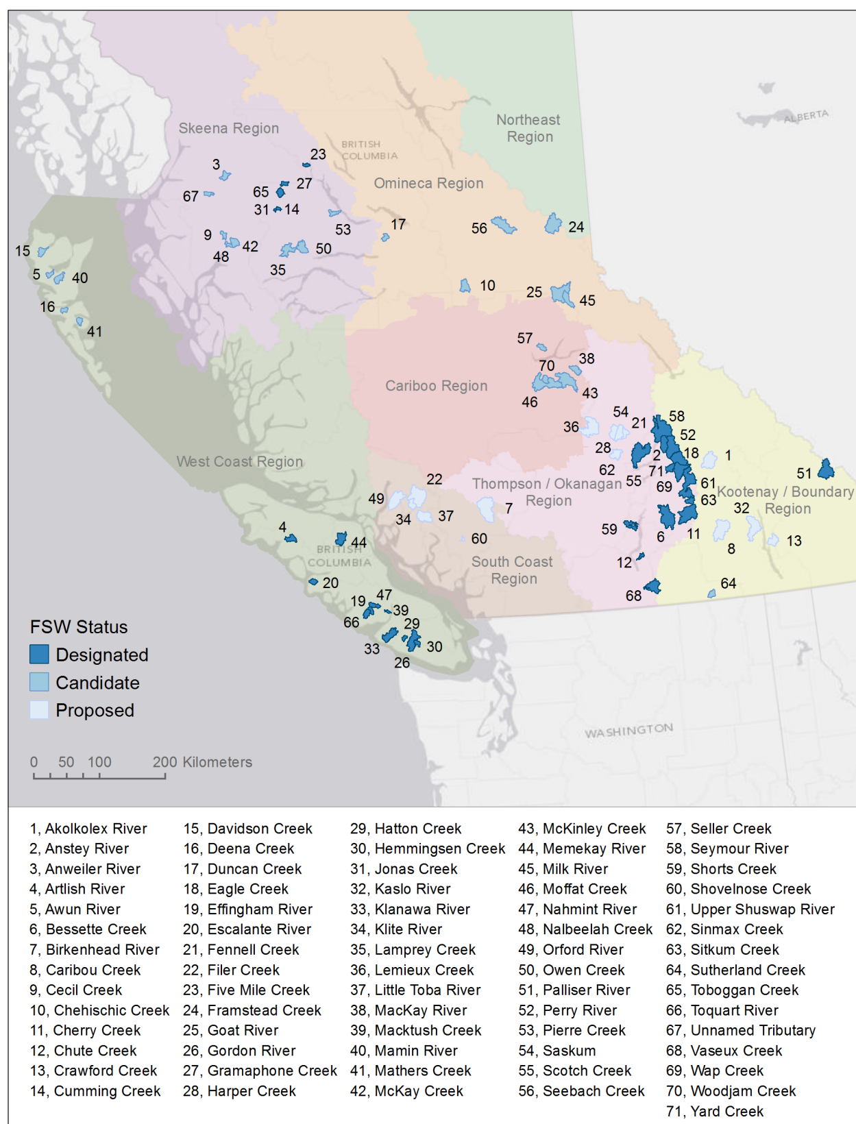
Figure 1. Location of 71 designated, candidate, and proposed fisheries sensitive watersheds within British Columbia's natural resource management regions.
