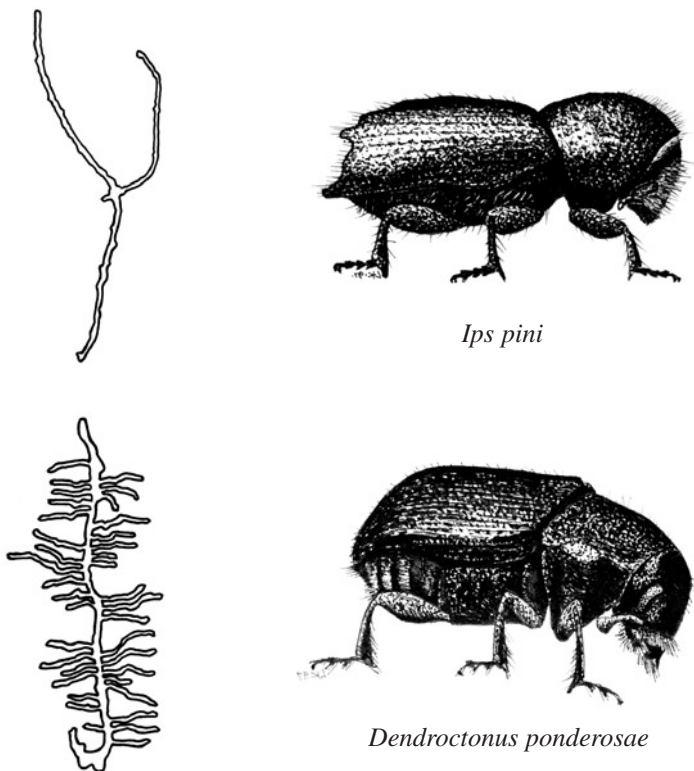
Figure 3. Diagram showing galleries and adults of Ips pini (top) and Dendroctonus ponderosae (bottom).
