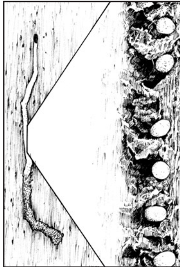
Figure 4. Mountain pine beetle parent gallery with inset showing eggs laid in niches.
