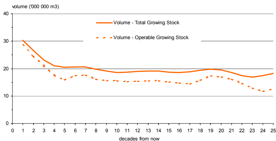
Figure 3-7 Total and operable growing stock, silviculture base case.
