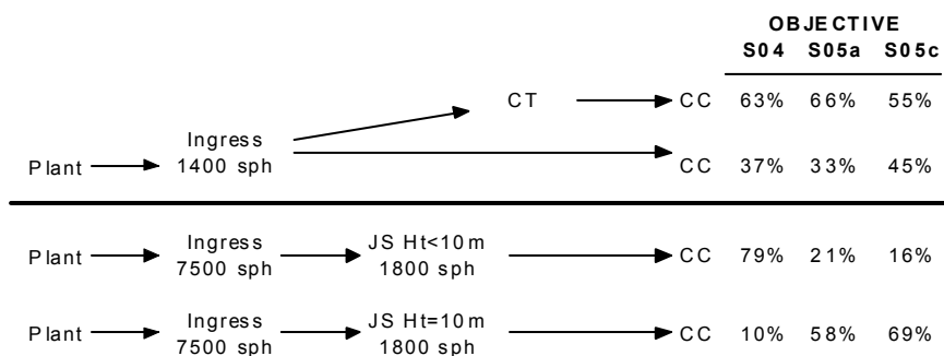
Figure 4-7 Dominant regimes for SAU03, all scenarios.
