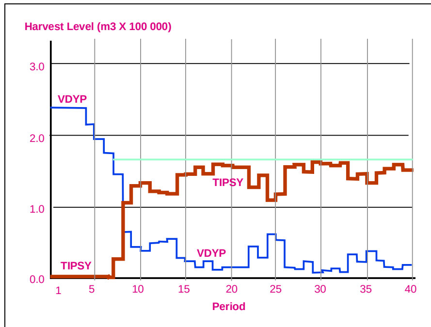
Figure 1. Harvest Queue of Existing Stands (VDYP) and Managed Stands (TIPSY)
