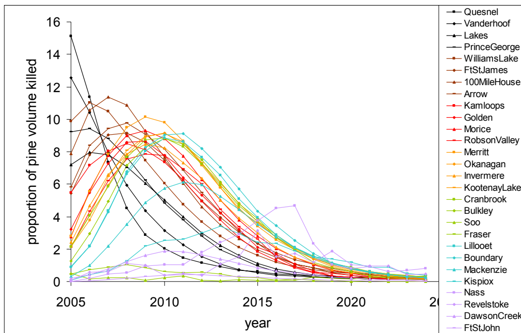
Figure 5. Effect of initial proportion of volume killed on the progression of the outbreak.
