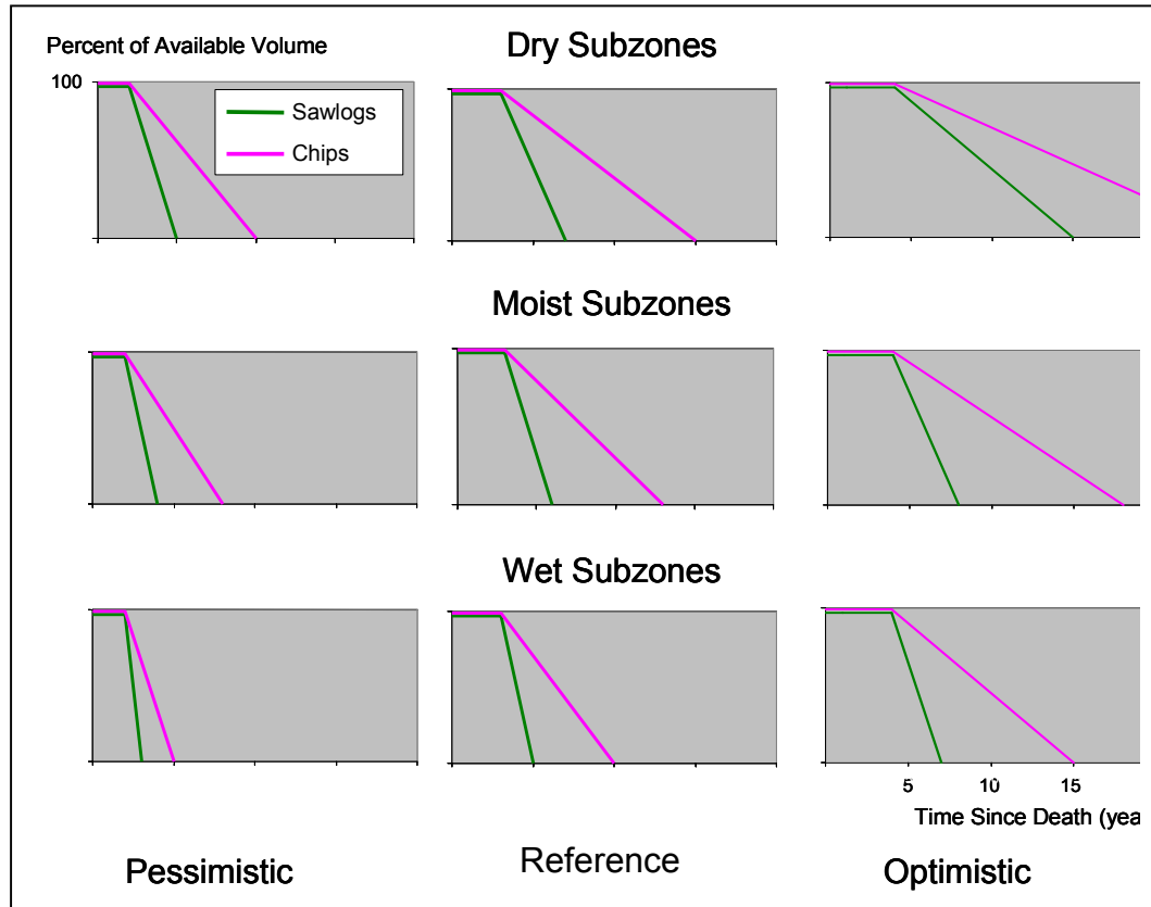
Figure 2. Relationship between time since death and the amount of volume available for the sawlog and “alternative” (chip) industries in dry, moist and wet subzones under pessimistic, reference and optimistic assumptions.
