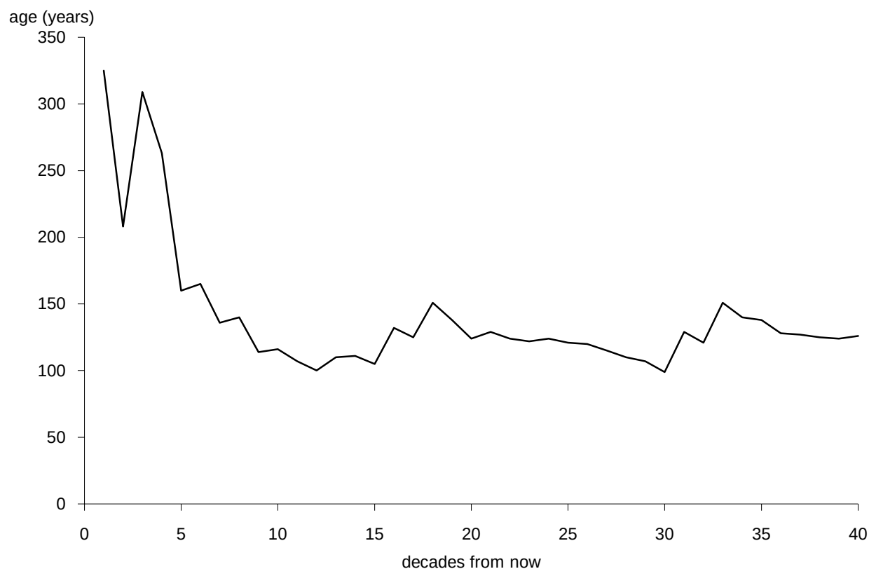
Figure 12. Average age harvested over time — Arrowsmith TSA base case, 1995.
