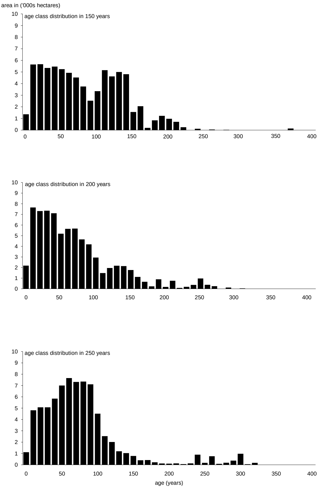
Figure 13. Stand age class composition over time — Arrowsmith TSA base case, 1995 (concluded).
