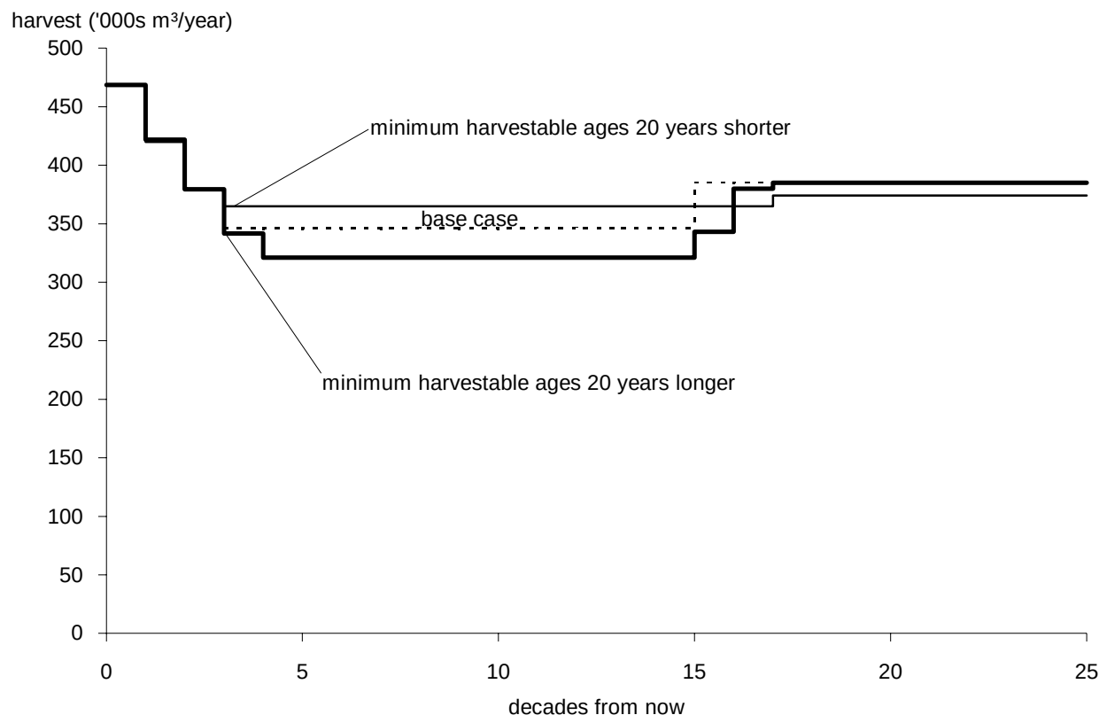
Figure 19. Harvest forecasts if minimum harvestable ages are 20 years different than the base case — Arrowsmith TSA 1995.
