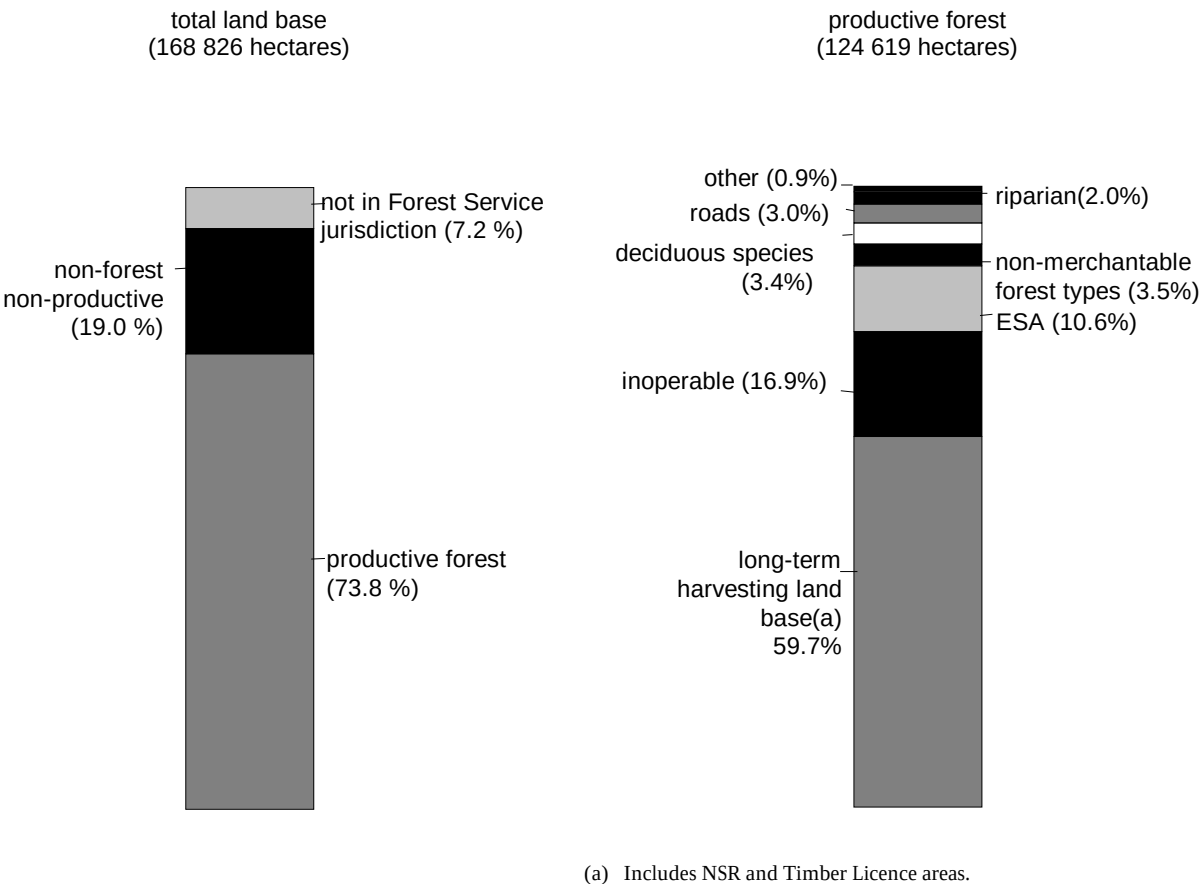
Figure 3. Classification of the total and productive forest land bases — Arrowsmith TSA, 1995.
