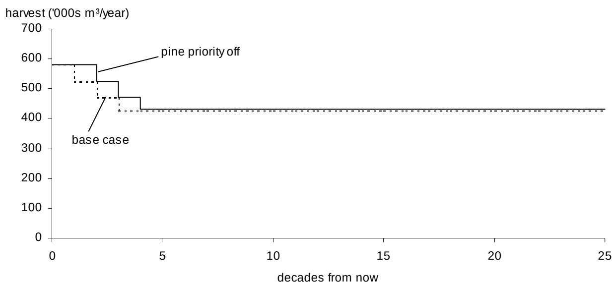
Figure 22. Forecasts showing effect of removing the pine priority — Invermere TSA, 2000.
