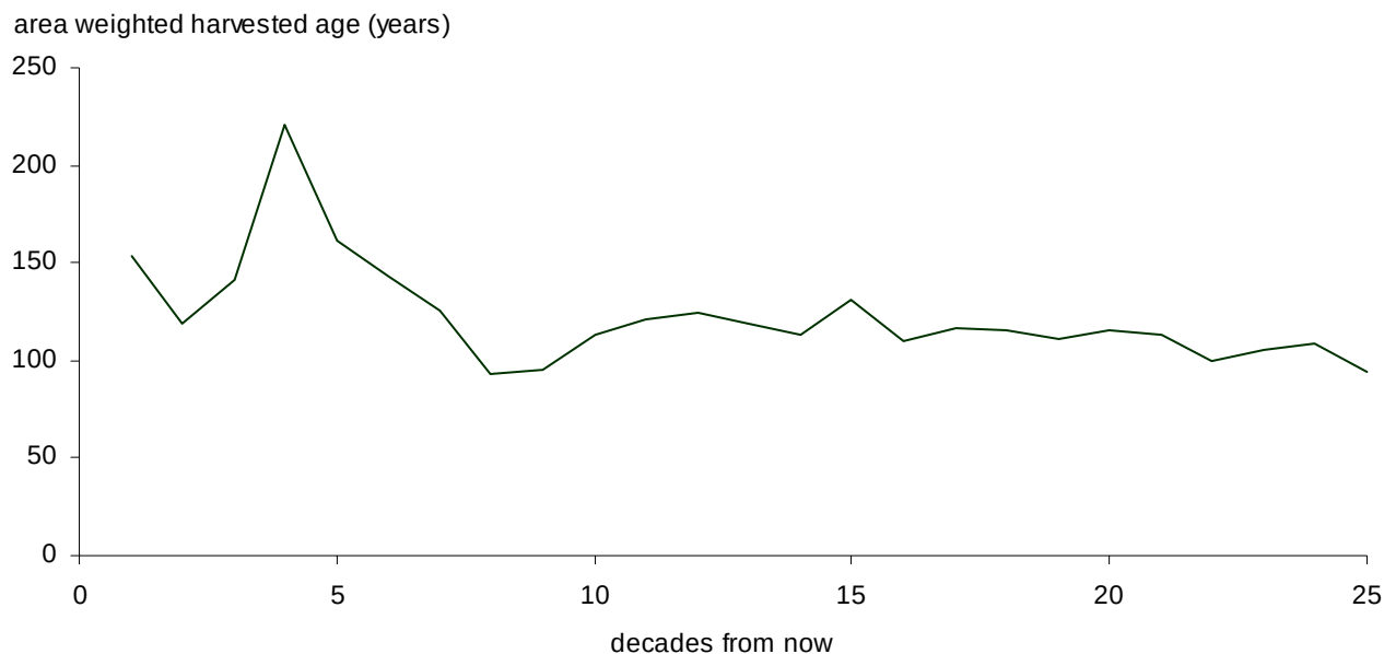
Figure 12. Average age of stands harvested over time — Invermere TSA base case, 2000.
