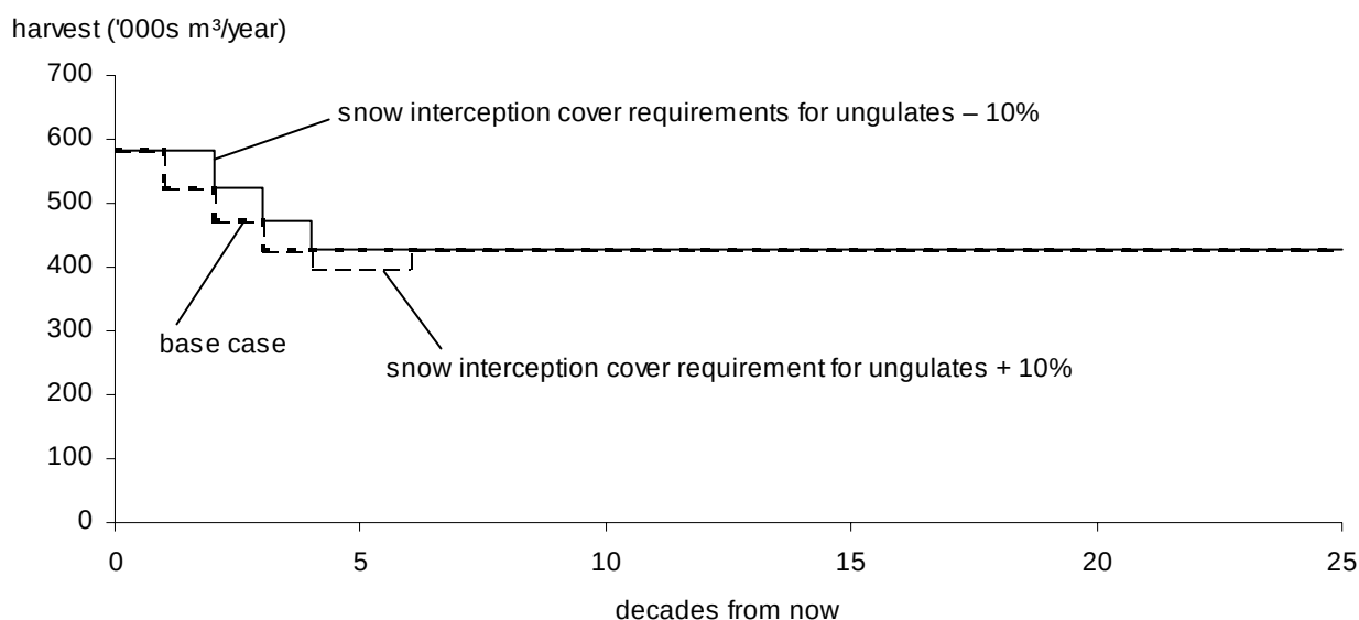
Figure 20. Harvest forecasts showing effects of changes to percentage snow interception cover required — Invermere TSA, 2000.
