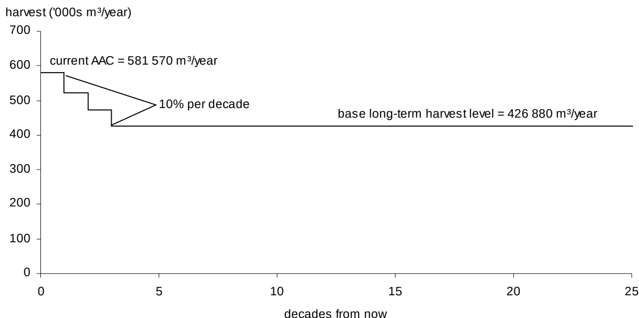
Figure 8. Base case harvest forecast for the Invermere TSA, 2000.
