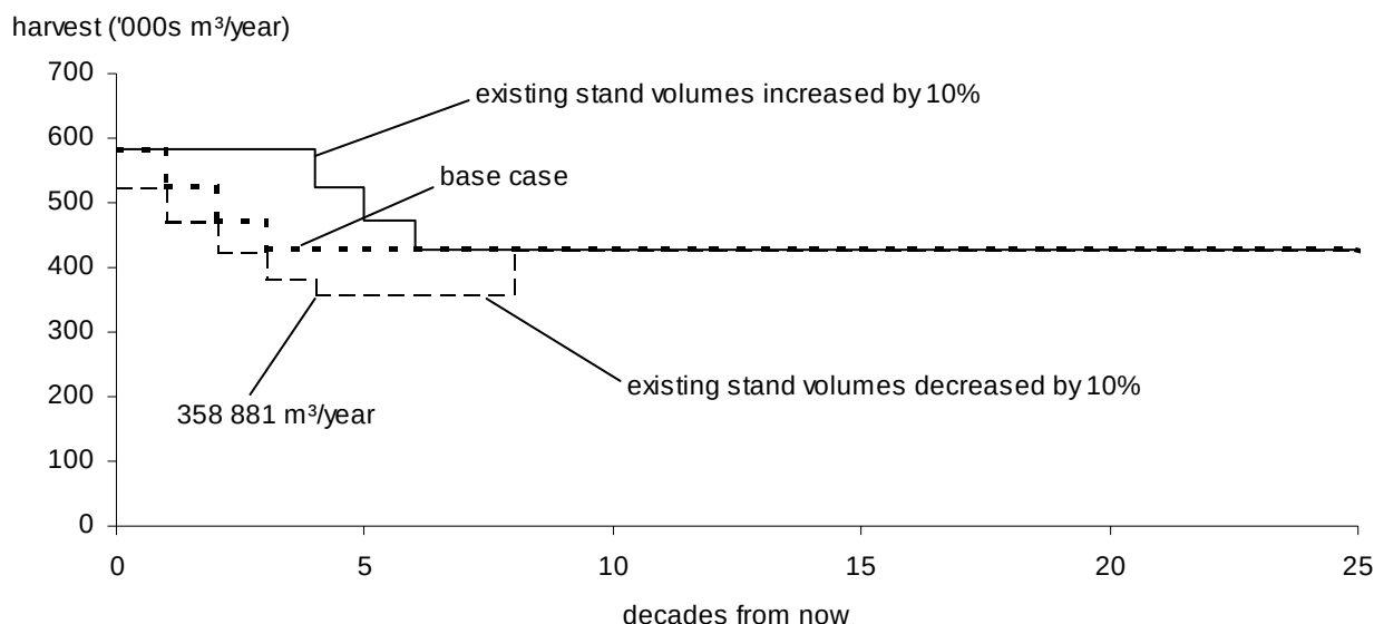
Figure 17. The effect on the harvest forecast of increasing and decreasing volume estimates for existing unmanaged stands by 10% — Invermere TSA, 2000.
