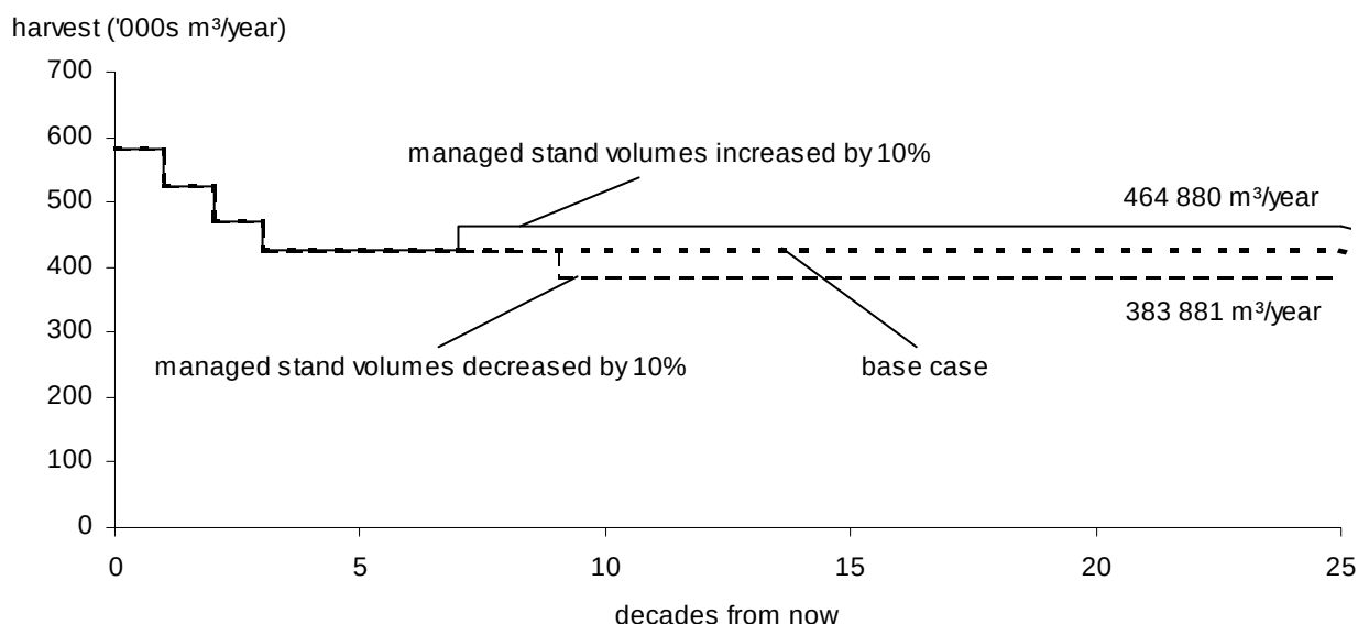
Figure 18. The effect on the harvest forecast of increasing and decreasing volume estimates for managed stands by 10% — Invermere TSA, 2000.
