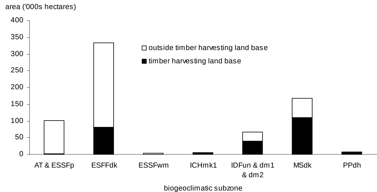
Figure 3. Forested area by biogeoclimatic classification — Invermere TSA, 2000.
