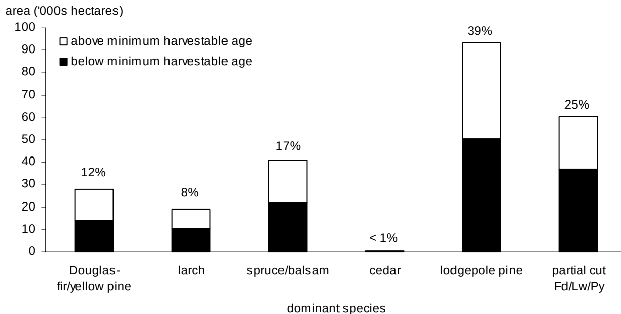
Figure 4. Area by dominant species — Invermere TSA timber harvesting land base, 2000.
