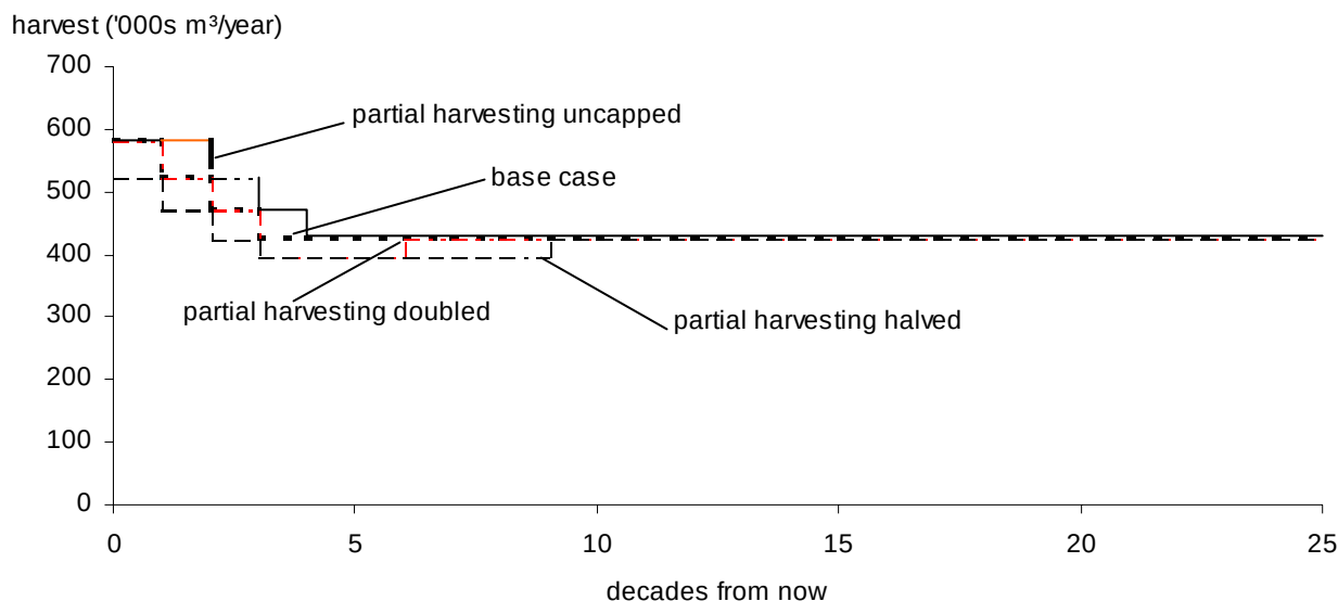
Figure 23. Forecasts showing effects halving, doubling and uncapping the partial harvest — Invermere TSA, 2000.
