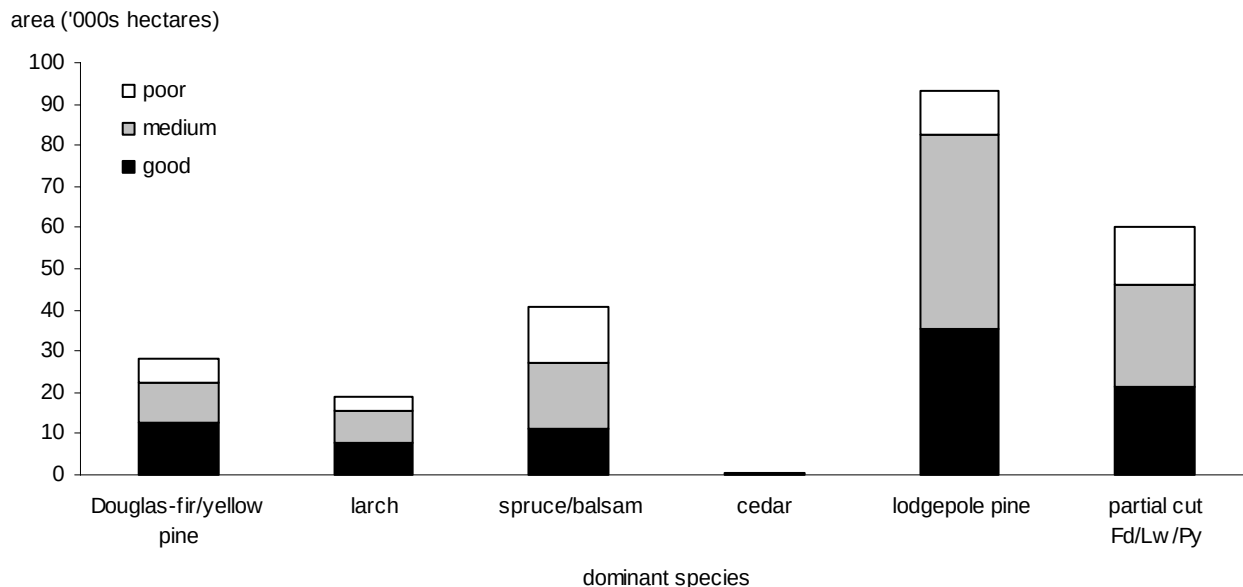
Figure 5. Area by predominant species and site productivity — Invermere TSA timber harvesting land base, 2000.
