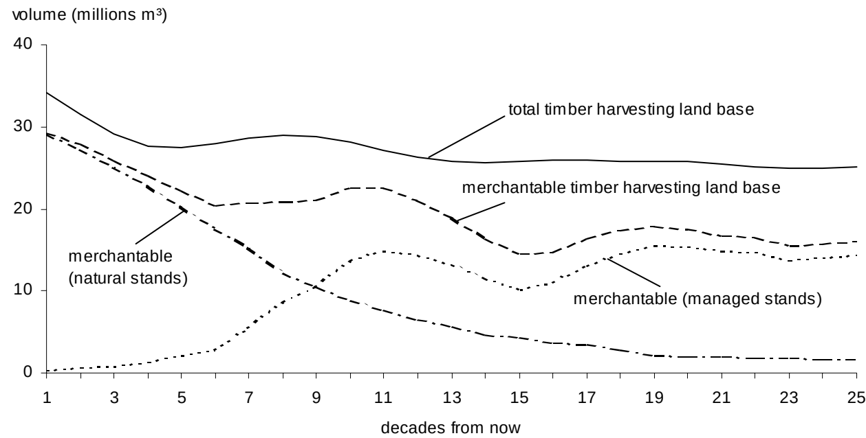
Figure 11. Total and merchantable growing stocks — Invermere TSA, 2000.
