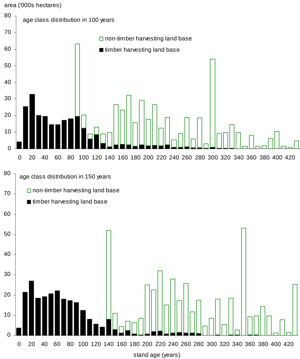
Figure 15. Changes in age distribution on the productive land base over time — Invermere TSA base case, 2000.
