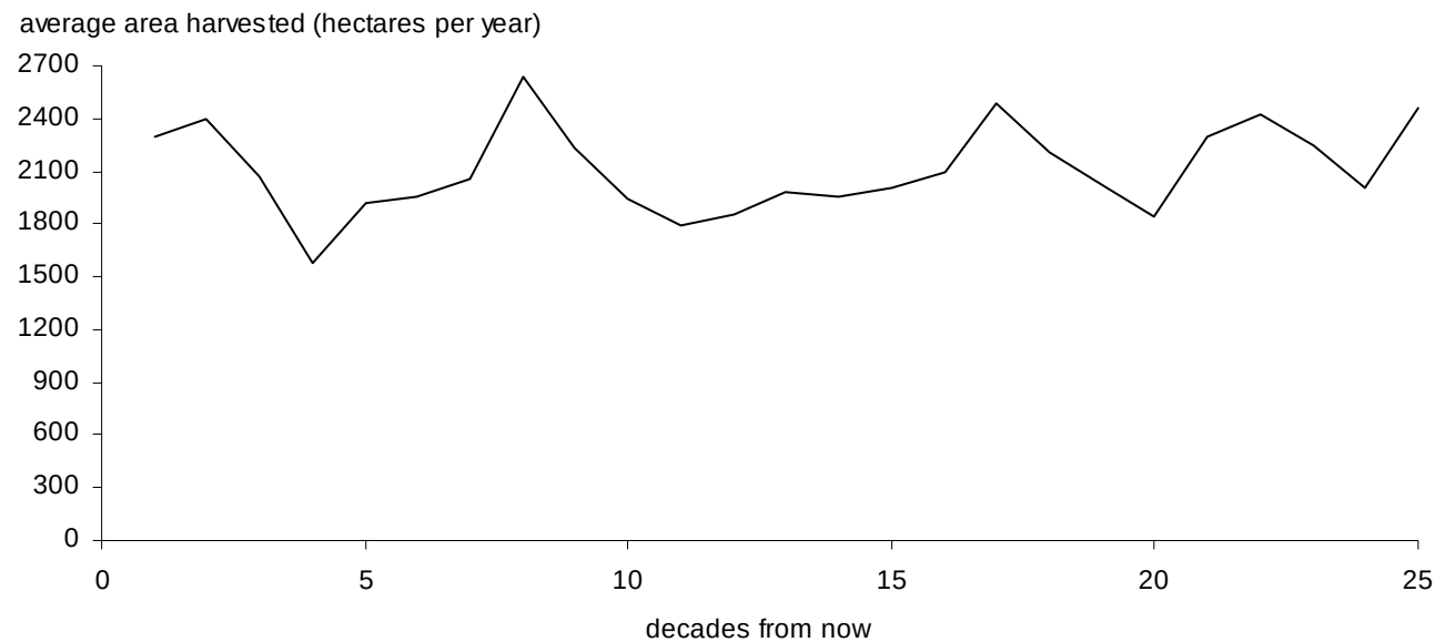
Figure 13. Average area harvested over time — Invermere TSA base case, 2000.
