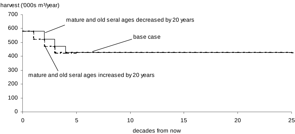
Figure 28. Harvest forecasts if landscape-level biodiversity age assumptions are changed — Invermere TSA, 2000.
