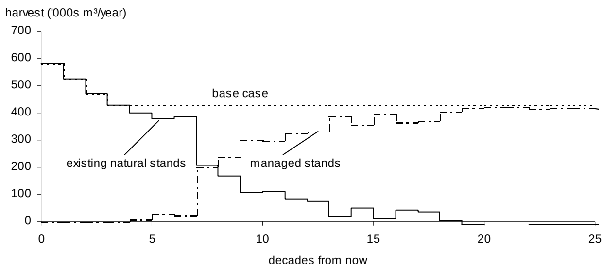
Figure 10. Harvest contribution from the unmanaged and managed stands — Invermere TSA, 2000.
