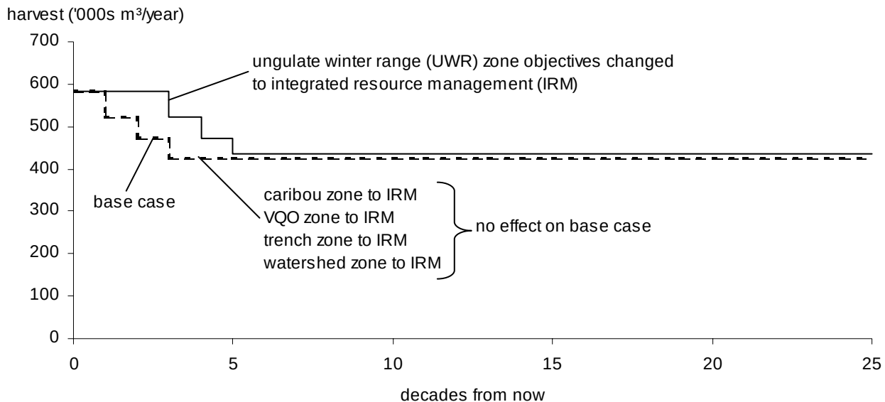
Figure 19. Harvest forecasts resulting when forest cover requirements for each zone are changed to IRM—Invermere TSA, 2000.
