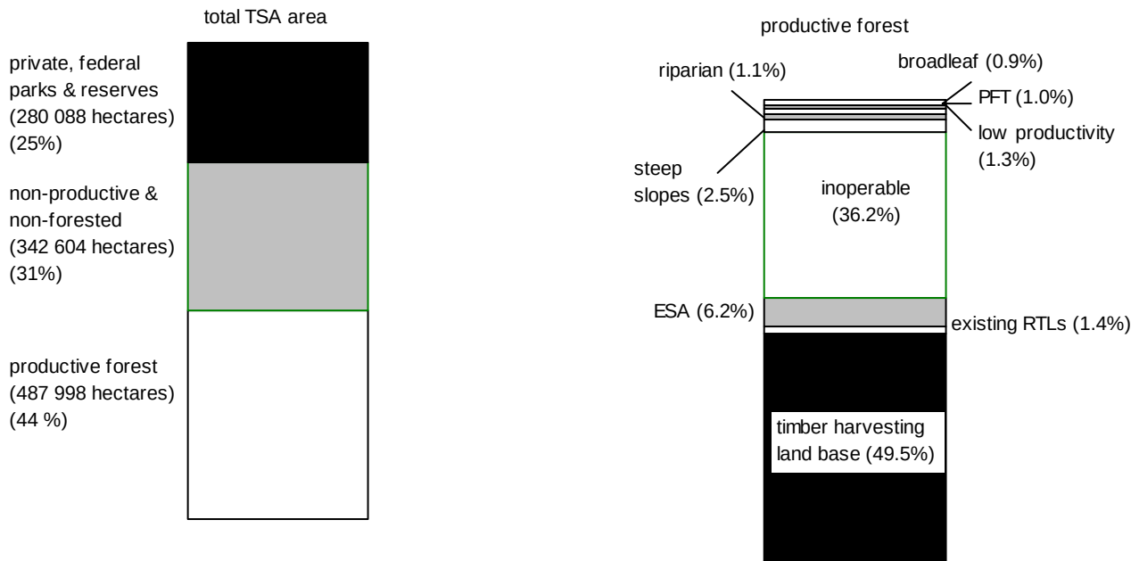
Figure 2. Composition of the total and Crown forested land bases — Invermere TSA, 2000.
