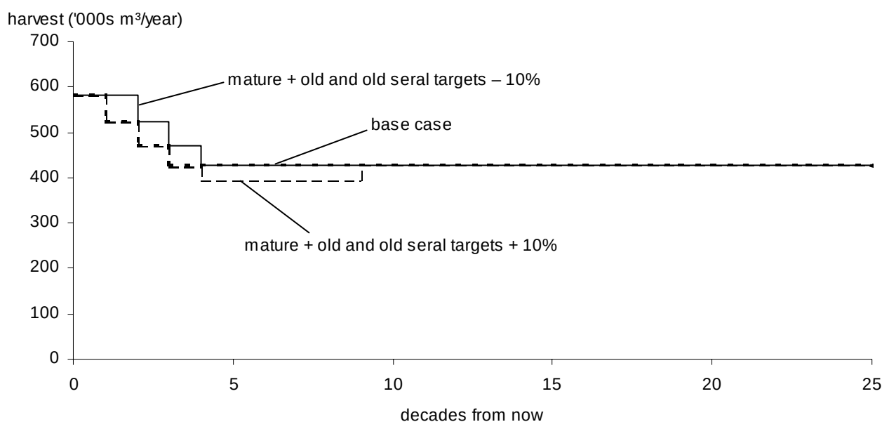
Figure 27. Harvest forecasts if landscape-level biodiversity mature and old seral* percentage requirements are changed — Invermere TSA, 2000.
