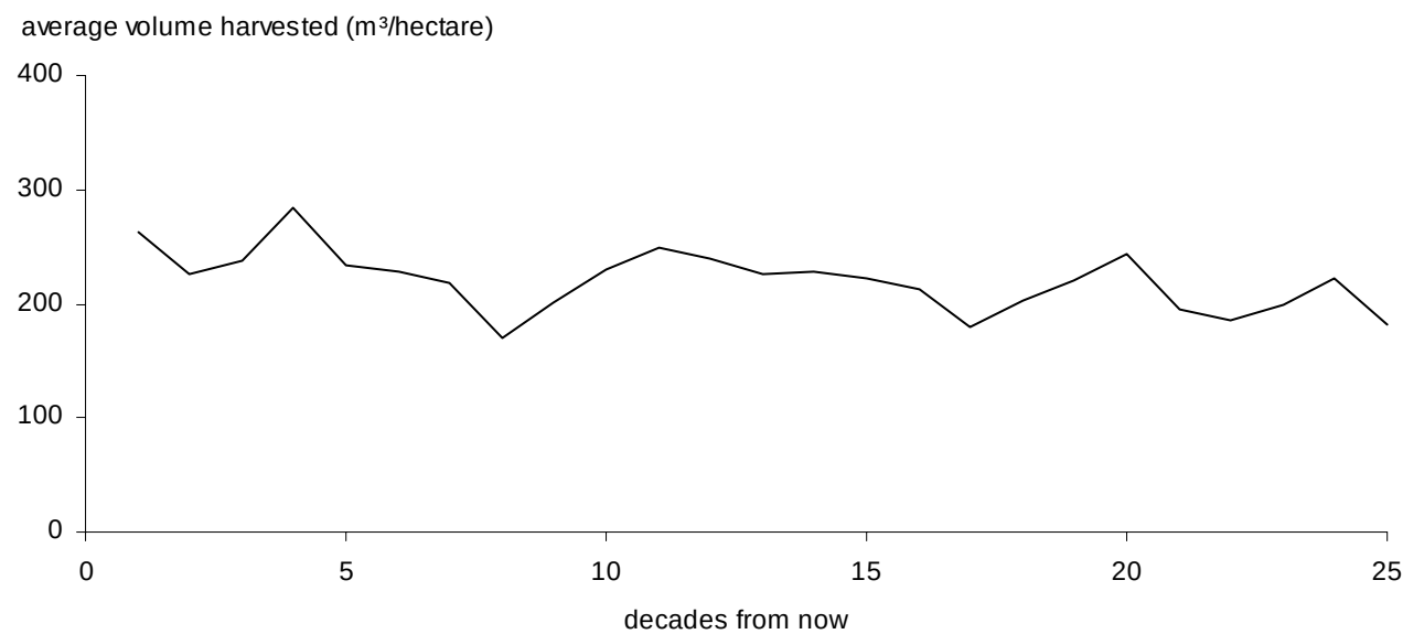
Figure 14. Average volume per hectare harvested over time — Invermere TSA base case, 2000.
