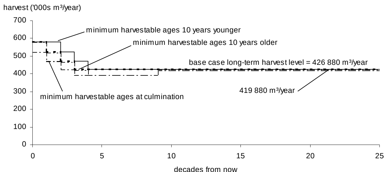
Figure 25. Harvest forecasts if minimum harvestable ages are younger or older than the base case — Invermere TSA, 2000.
