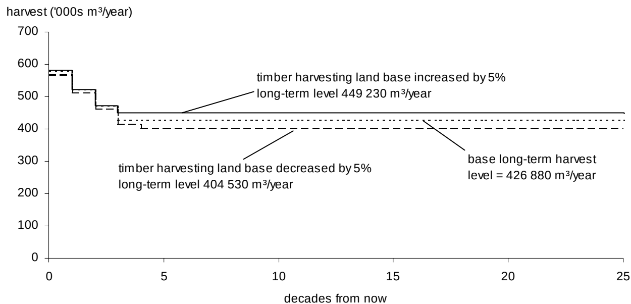
Figure 16. Land base sensitivity analysis — Invermere TSA, 2000.
