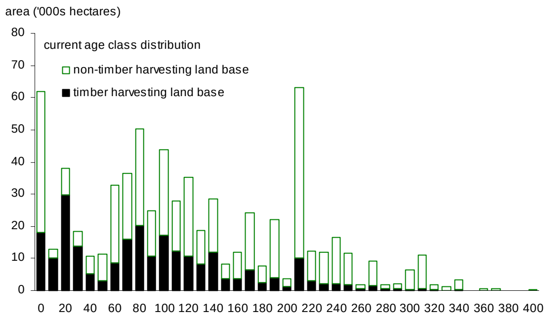
Figure 6. Current age class distribution — Invermere TSA forested land base, 2000.
