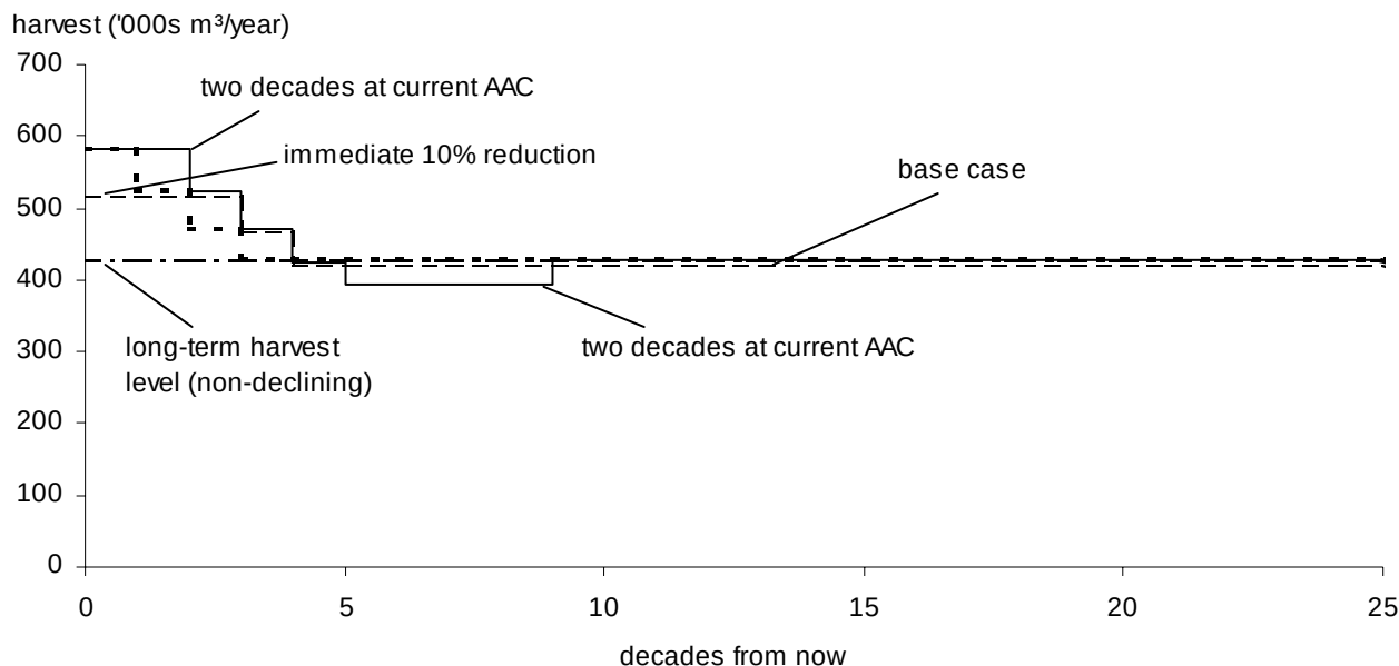
Figure 9. Alternative harvest flows — Invermere TSA, 2000.
