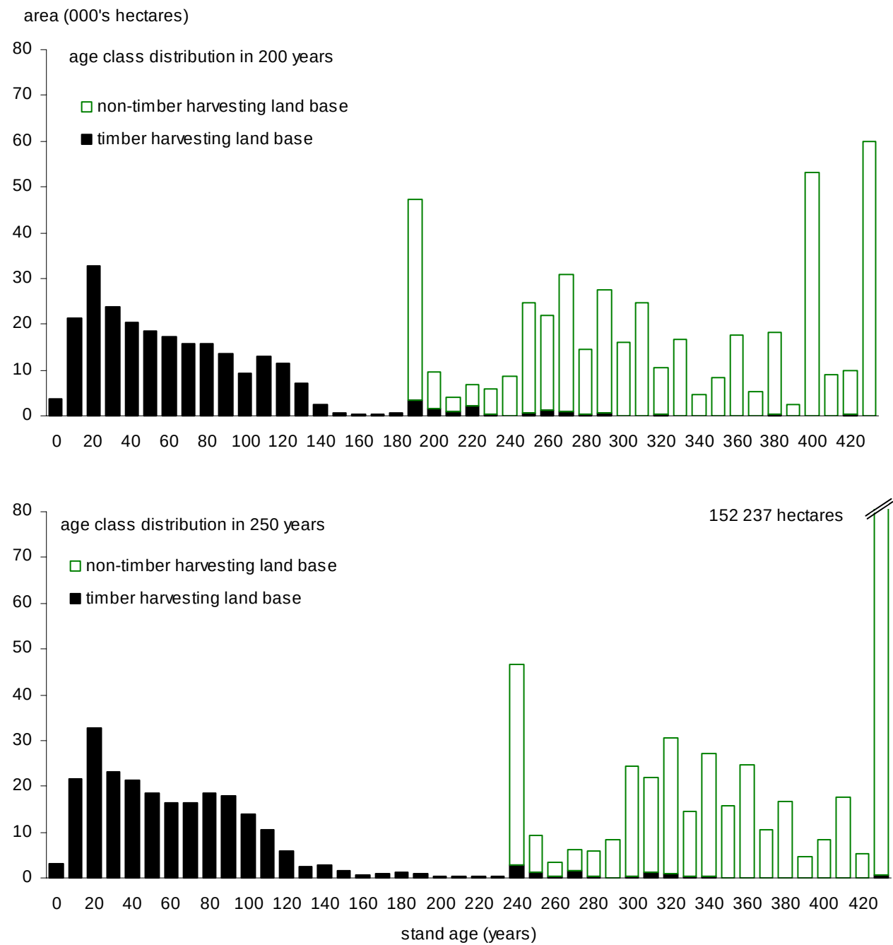
Figure 15. Changes in age distribution on the productive land base over time — Invermere TSA base case, 2000.
