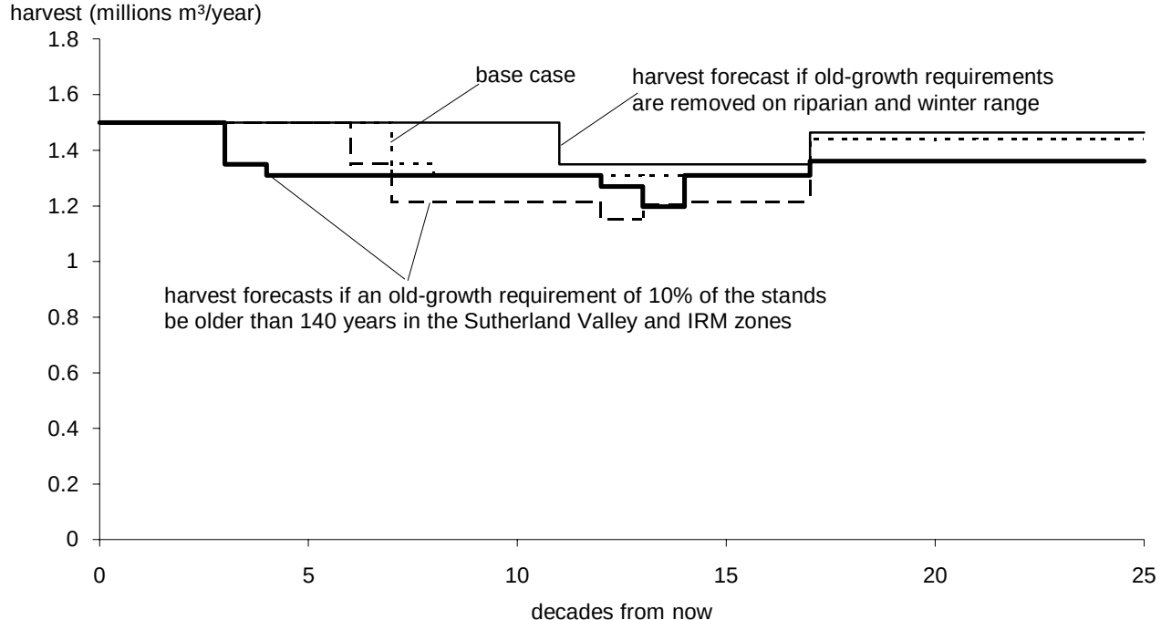
Figure 21. Harvest forecasts if the forest cover objectives for old growth were different than the base case — Lakes TSA, 1995.
