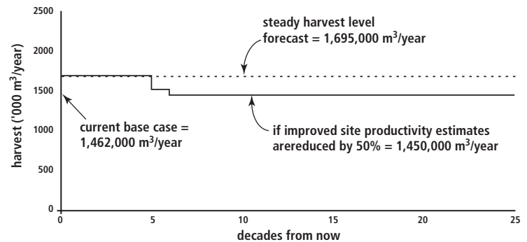
Figure 6. Uncertainty about site productivity estimates for managed pine stands, Lakes TSA, 2001.
