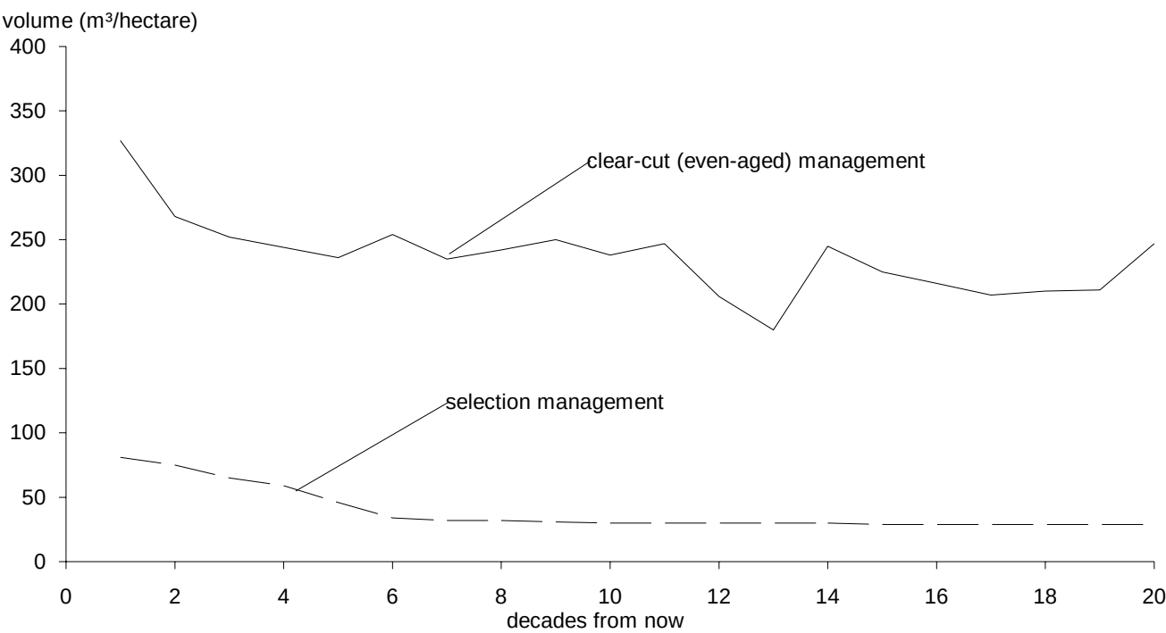
Figure 13. Average volume per hectare harvested over time, base case.
