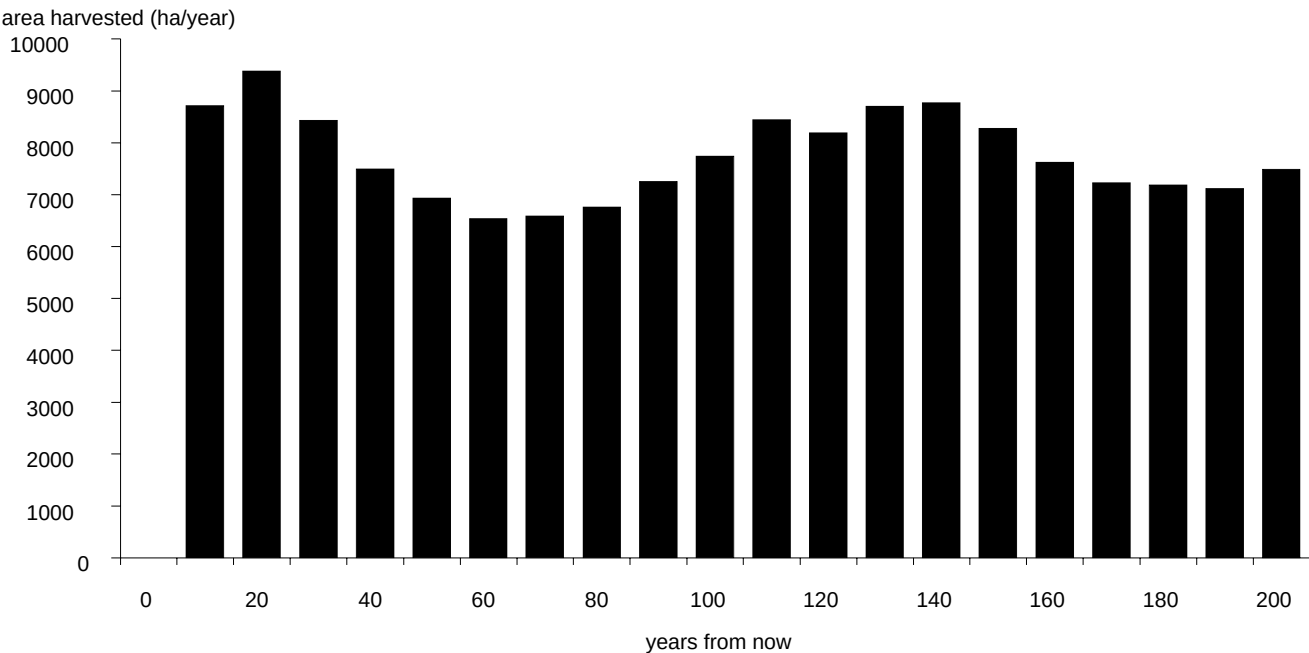
Figure 8. Area harvested annually for base case.
