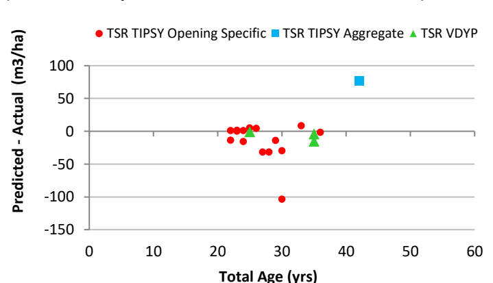
Total volume bias at each YSM location (Predicted TSR yield table volume - Actual YSM volume)
