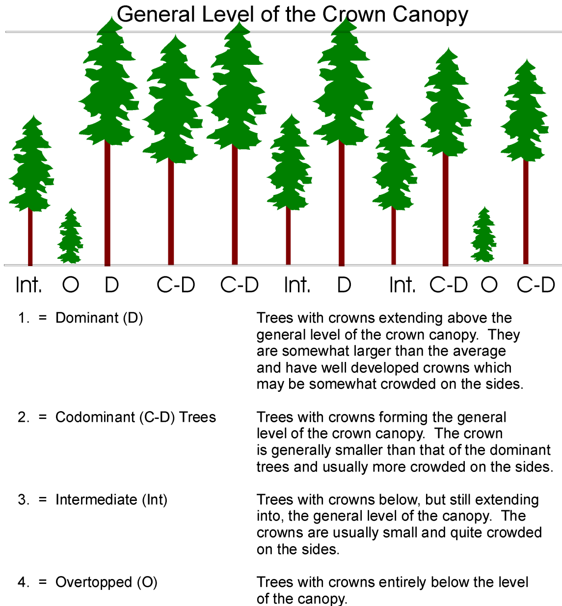
Figure 3.9 Crown classes.
