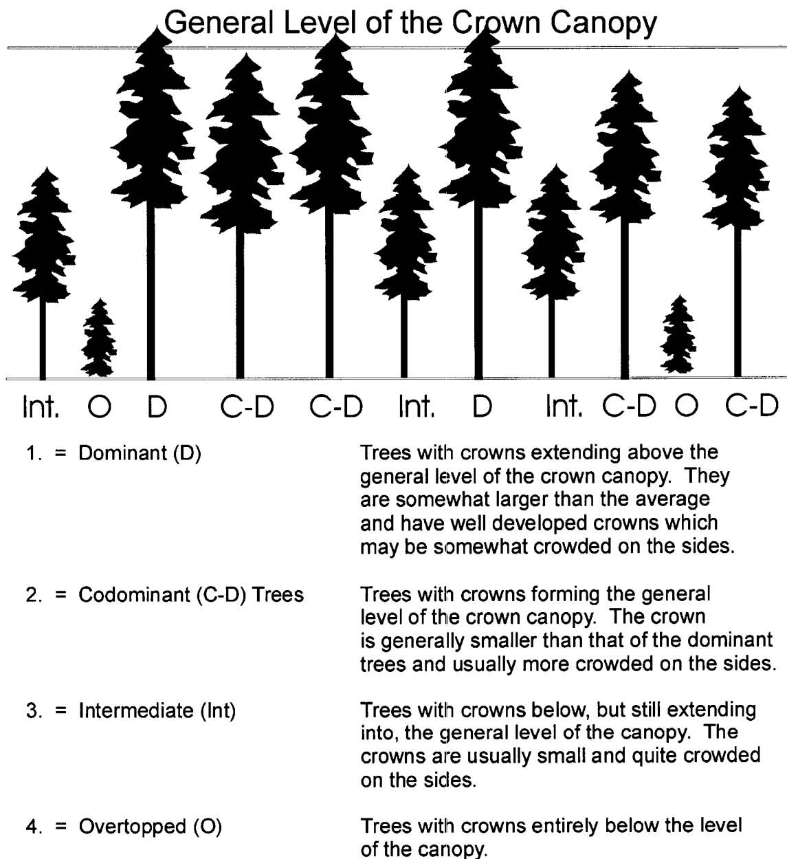
Figure 3.10 Crown classes.
