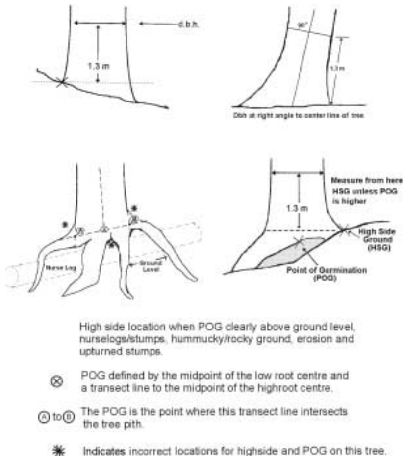
Figure 3.12 DBH in relation to high side.
