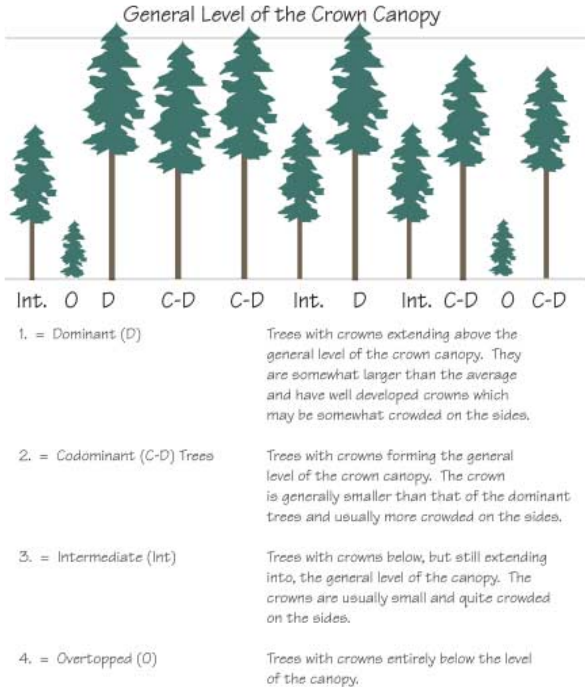
Figure 3.13 Crown Classes.
