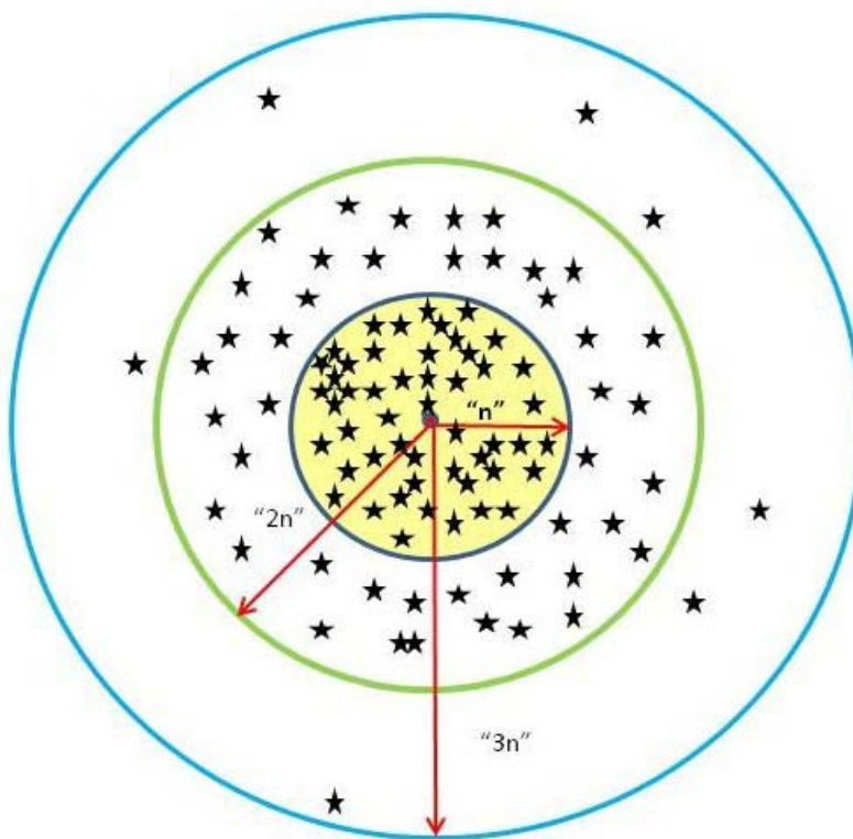
Figure A.2 Circular Error Probability
