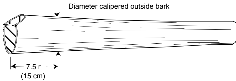
6.24 Measuring diameter for interior undersize grade.
