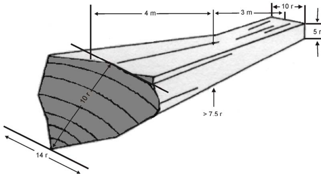
Figure 8.20 Slabs with Portions Meeting the Grade Rule.
