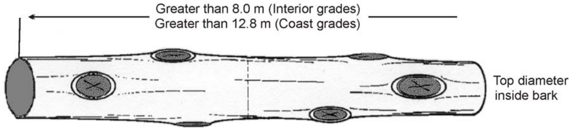
Figure 8.9 Knots and Midpoint.
