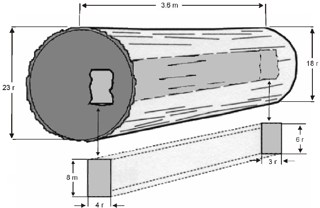
Figure 7.10 A Log with Through-running Pocket Rot.
