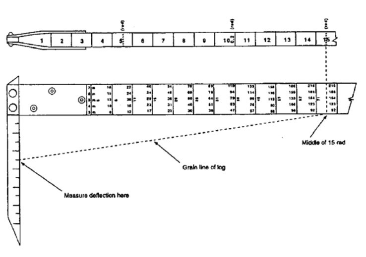
Figure 8.5 Measuring Twist – Reading the Deflection.
