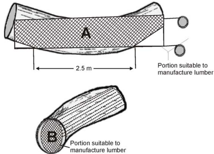
Figure 8.54 Using a Tape to Evaluate Sweep in Logs or Sections From the Sides (A) or From the Ends (B) of the Log.
