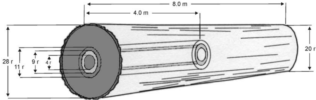
Figure 8.32 Only the Collar Meets the Grade Rules.
