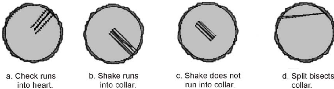
Figure 8.40 Trim Allowance for Check, Shake and Split in Relation to Collars.
