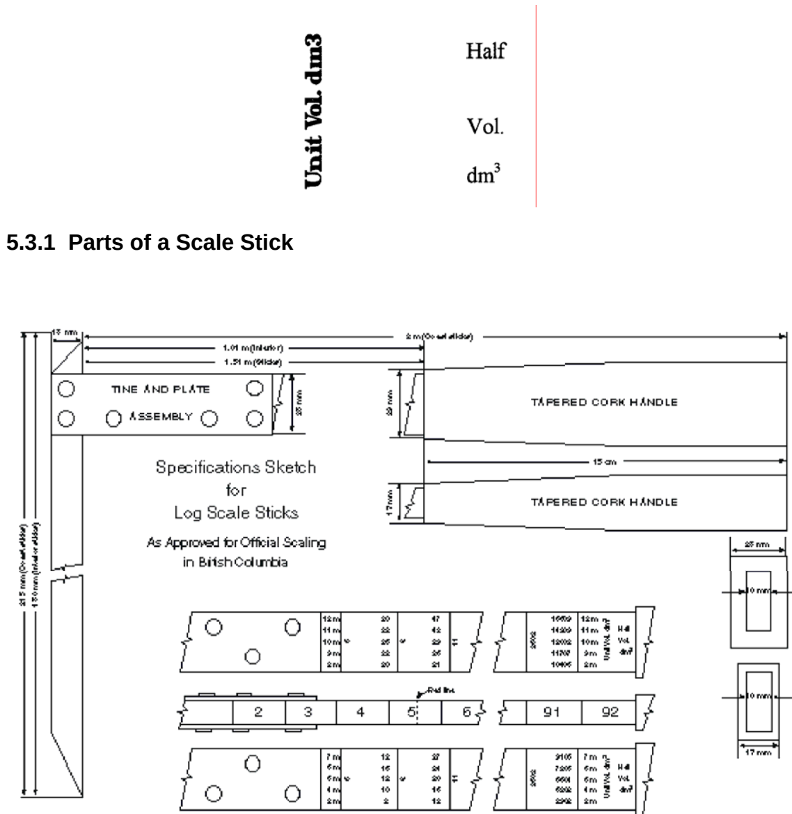
Figure 5.9 BC Metric Log Scale Stick – Specifications Sketch.
