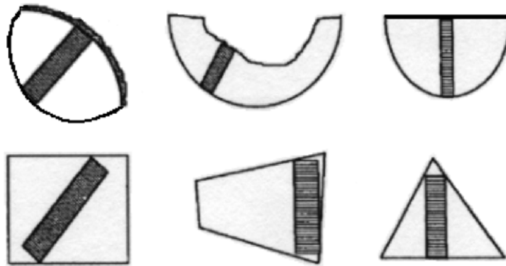
Figure 8.21 Maximum Thicknesses at Right Angles to the Grain.
