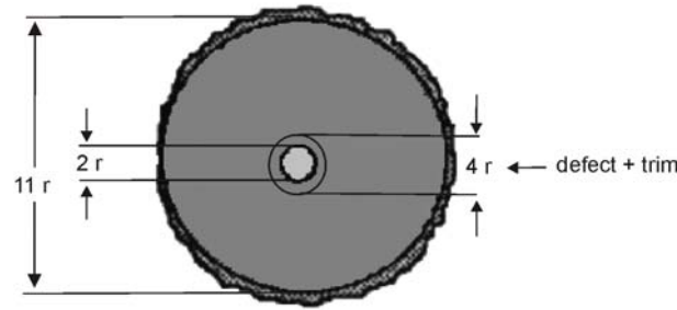
Figure 8.24 Trim and the Twenty Percent Rule.
