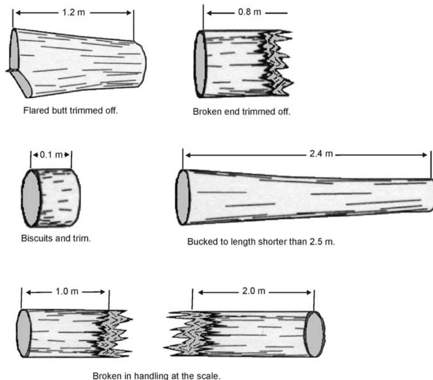
Figure 8.50 Examples of Short Logs Left After Bucking at the Scale Site and Deemed to be 2.5 m Long (Interior) and 5.2 m Long (Coast).
