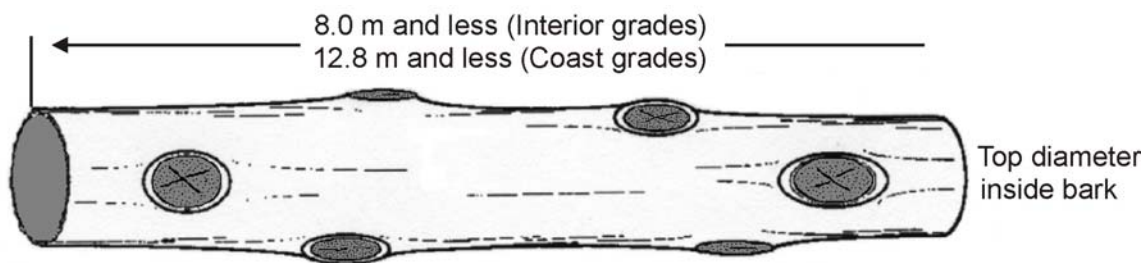
Figure 8.8 Assessing Knots - Coast and Interior.
