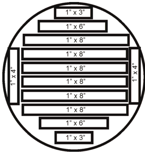
Figure 8.1 Lumber Definition from the NLGA.
