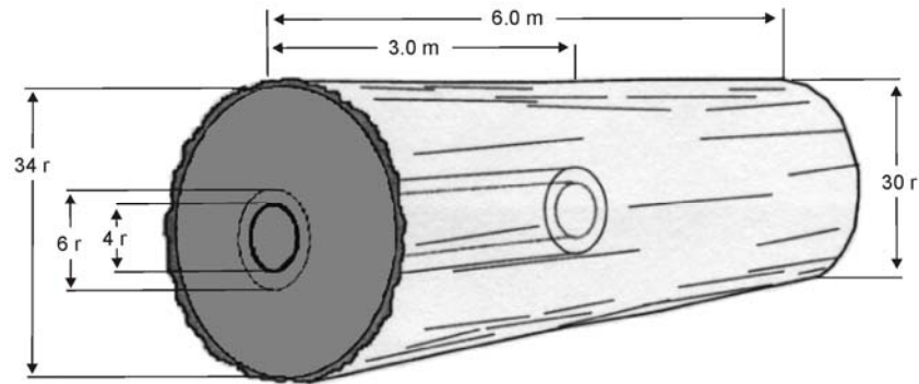
Figure 8.30 Ring Shake and Only the Collar is Thick Enough to Produce Lumber.
