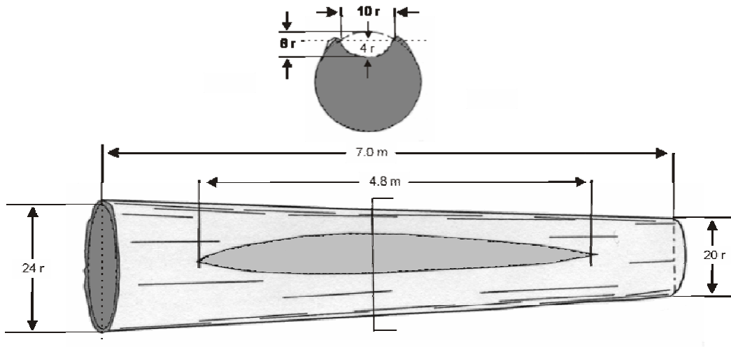
Figure 7.5 A Log with a Double Conical Catface.
