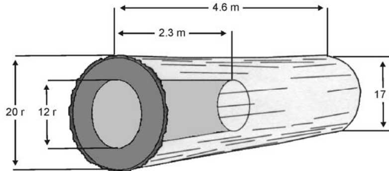
Figure 8.49 Assessing Grade in Log with Severe Heart Rot and Residual Length is Too Short to Cut Lumber.
