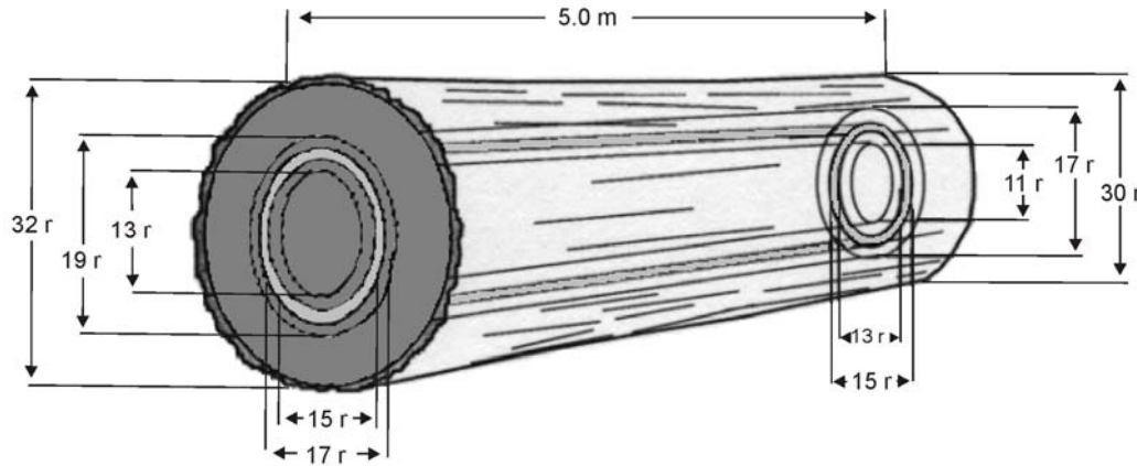
Figure 8.31 Both Core and Collar Meet the Grade Rule.
