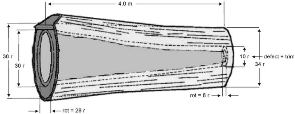
Figure 8.26 Through Running Butt Rot.
