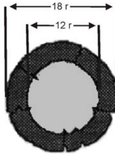
Figure 8.17 Advanced Sap Rot.
