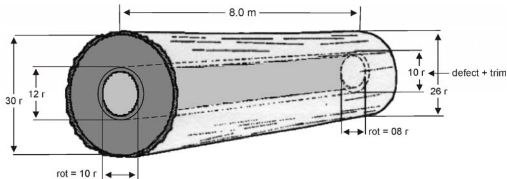
Figure 8.22 The Application of Trim Allowance Around Heart Rot and Hole.
