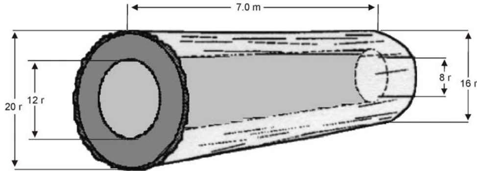
Figure 8.23 Collar Too Thin to Cut Lumber.
