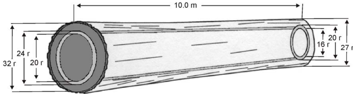
Figure 8.33 Only the Core Meets the Grade Rule.
