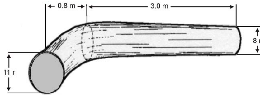
Figure 8.55 Visually Bucking a Log with Pistol Grip to Assess Lumber Recovery.
