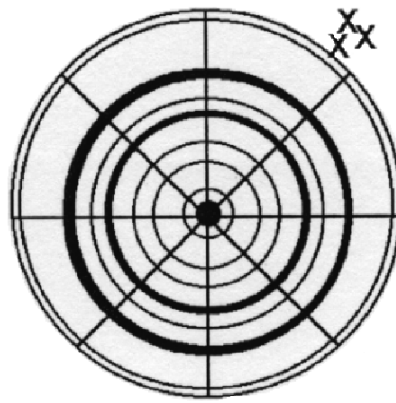
Figure 13.4 In this Dartboard Example, the 3 Darts (x) are Precise but Inaccurate and Biased.
