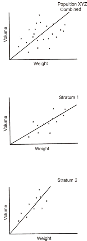
Figure 13.5 Graphs to Show the Impact of Stratification.
