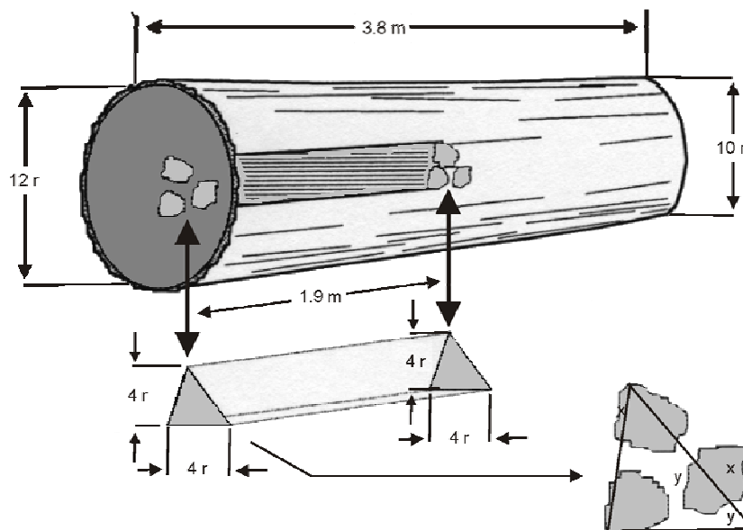
Figure 7.12 A Log with Partial-length Triangular Defect.
