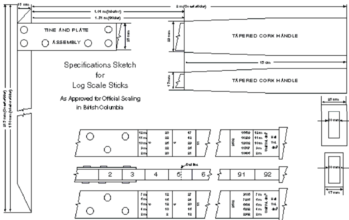
Figure 5.9 BC Metric Log Scale Stick – Specifications Sketch.
