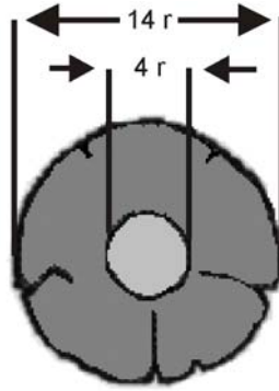
Figure 8.20 Residual Core is a Grade Reduction.
