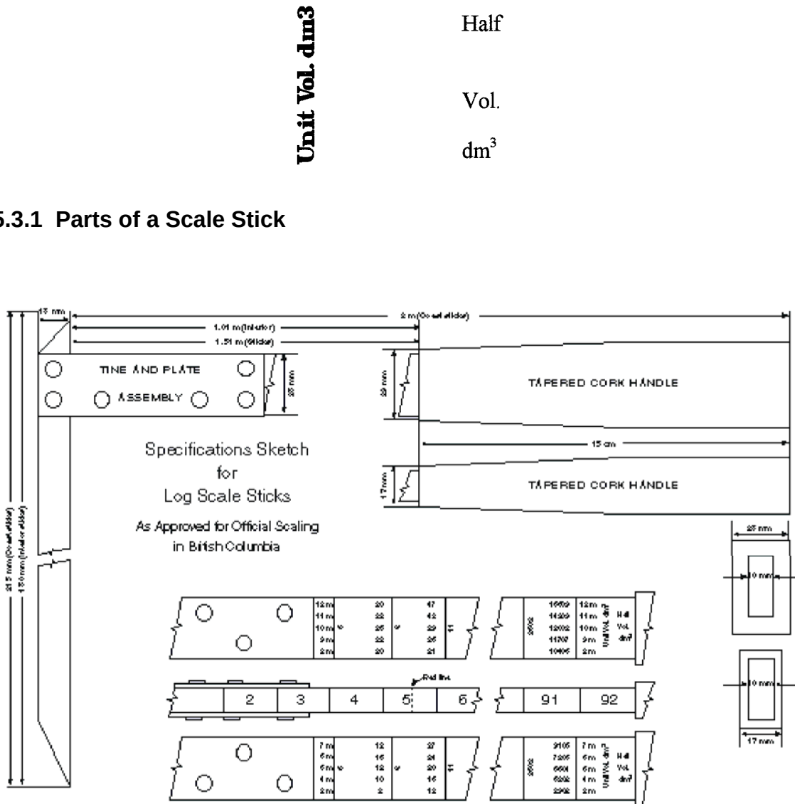
Figure 5.9 BC Metric Log Scale Stick – Specifications Sketch.
