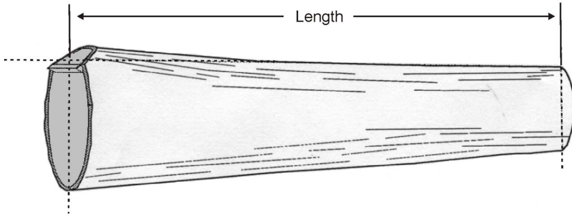
Figure 6.7 Length Measurement of Logs with Undercut.
