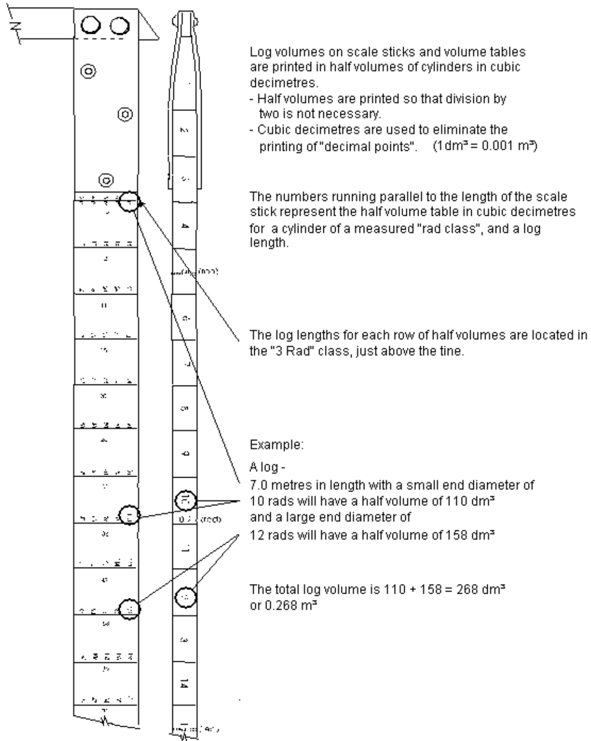
Figure 5.5 Using the BC Metric Scale Stick to Calculate Half Volumes.
