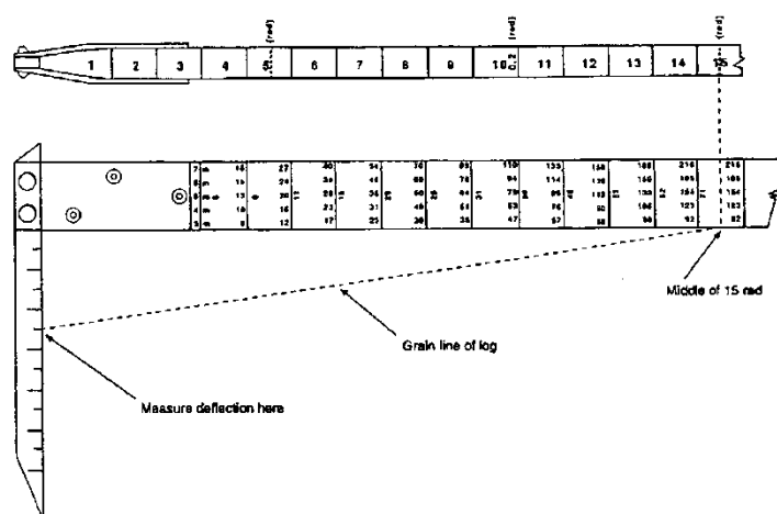
Figure 8.6 Measuring Twist – Reading the Deflection.
