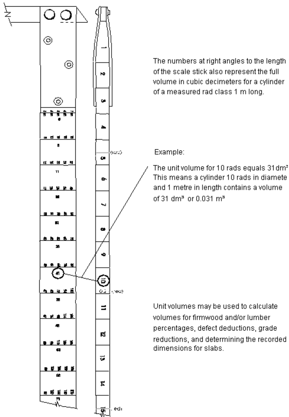
Figure 5.7 Obtaining Unit Volumes (or “factors” from the Scale Stick.
