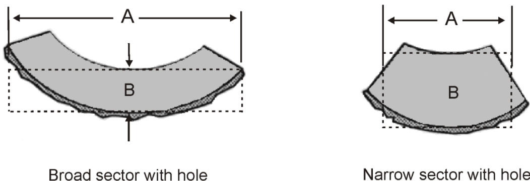
Figure 6.18 Measurement of a Sector Slab End with Hole.
