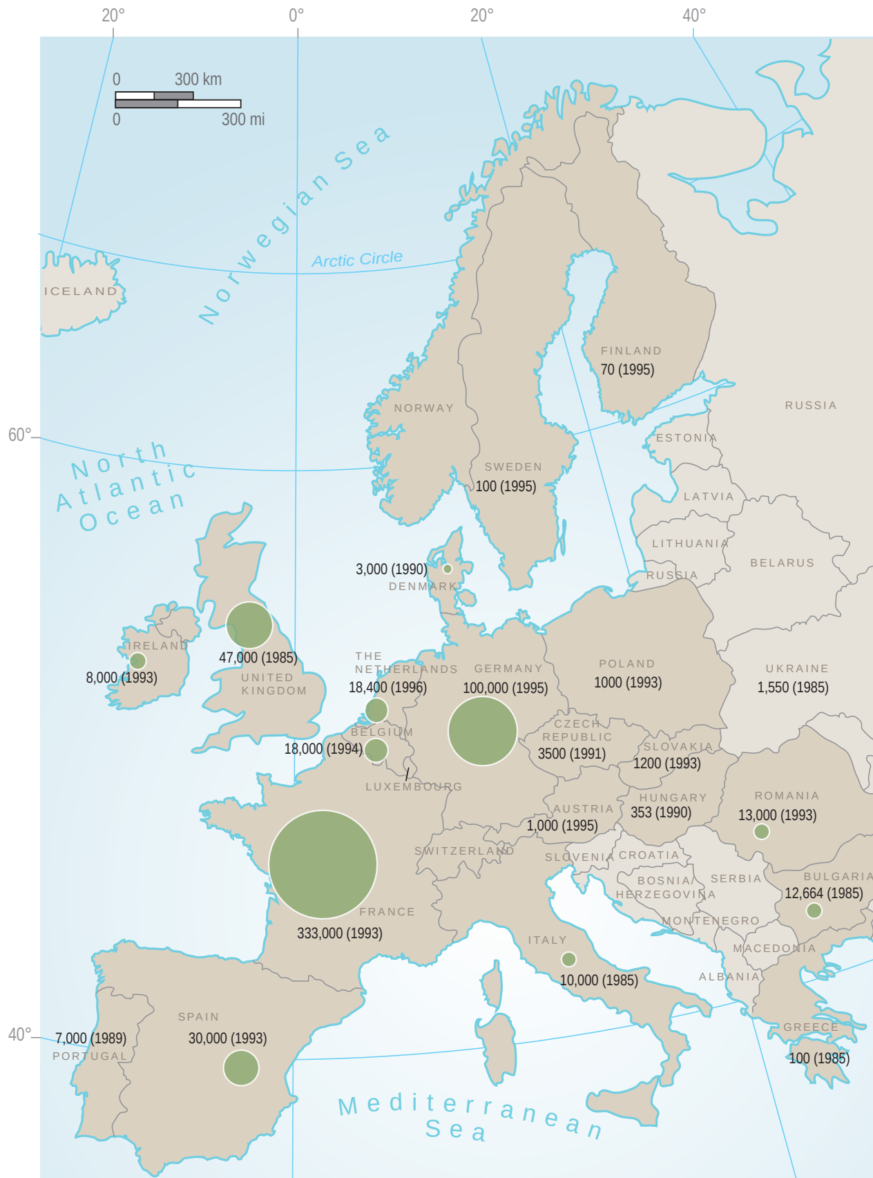
Figure 3.1 Areas occupied by Douglas-fir in Europe, in hectares (modified from De Champs 1997b). Some smaller stands or plantings may not be shown on this map, but may be discussed in the text or may appear on individual country maps.
