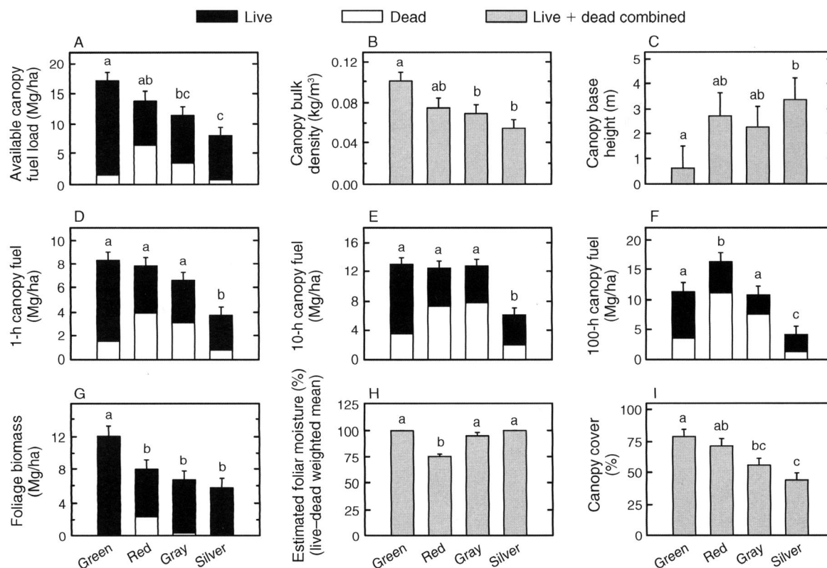
FIG. 4. Canopy fuels in each time-since-outbreak (TSO) class (green, red, gray, and silver). Bars represent basal-area-corrected mean values (i.e., the response value at the mean basal area) and standard errors from the general linear model (GLM). Lowercase letters are results of Tukey-Kramer pairwise comparisons among groups ( \alpha = 0.05 ), after accounting for variation in pre-outbreak conditions (basal area). See Appendix B for full statistical outputs from the GLM for all variables, including live/dead subcomponents. Fuel size classes are standard time-lag classes: 1-h fuels, <0.64 cm diameter; 10-h fuels, 0.64 – 2.54 cm; 100-h fuels, 2.54 – 7.62 cm. Note that estimated canopy foliar moisture is a weighted average including all live and dead foliage within a stand; for separate abundances of live and dead tree crowns, see Table 2.
