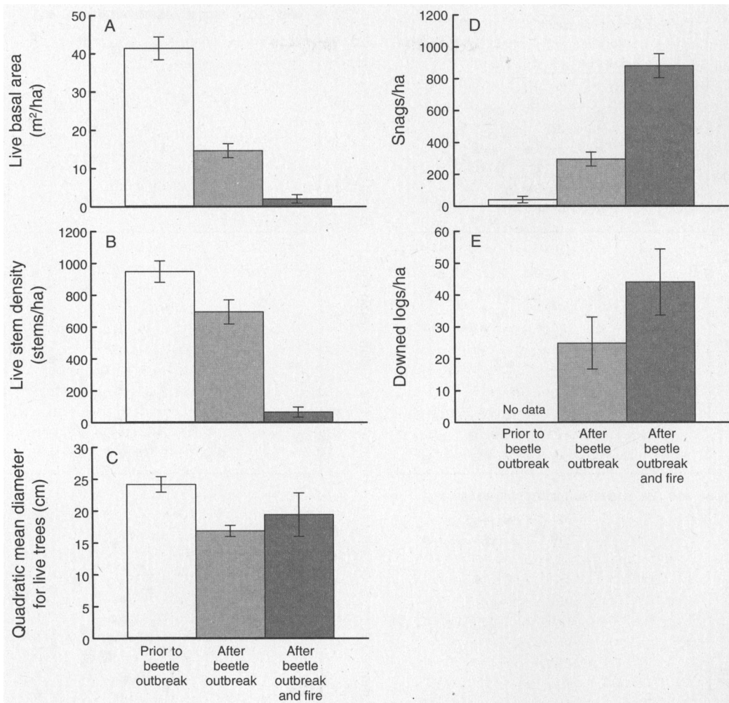
FIG. 1. Stand structure characteristics in all plots ( n = 85 ) prior to the bark beetle outbreak, after the bark beetle outbreak, and post-outbreak and postfire. Pre-outbreak values were reconstructed by assigning all trees killed by the fire and any trees with evidence of recent prefire beetle mortality as alive prior to beetle outbreak (Appendix B). Downed logs prior to beetle outbreak were not estimated because of decay over more than 10 years before sampling and possible combustion of some downed logs in the fire. Values are means and 95% confidence intervals.
