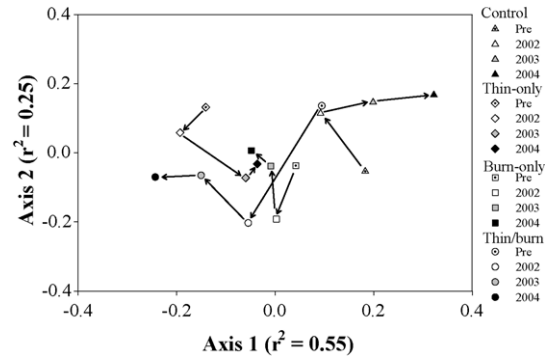
Fig. 4. NMS ordination of the understory plant community at the Lubrecht Forest FFS site before treatment and in the three subsequent years. Individual species covers were aligned to the block median cover (for each species) before analysis.
