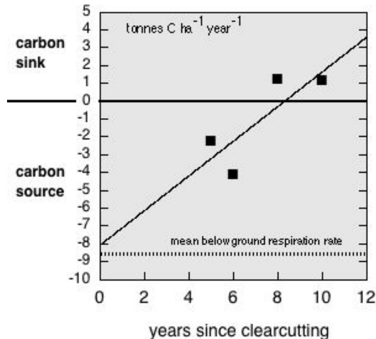
Figure 2. Transition from carbon source to carbon sink in a clearcut at the Aleza Lake Research Forest 60 km east of Prince George, British Columbia. Data are indicated for years 5, 6, 8, and 10 after clearcut harvesting. A linear regression line was fit to the relationship of annual forest-level net CO 2 exchange: NCE (tonnes C ha -1 y -1 ) versus clearcut age (years): NCE = 0.972 * (\text{clearcut age}) - 8.047 ; R^2 = 0.67
